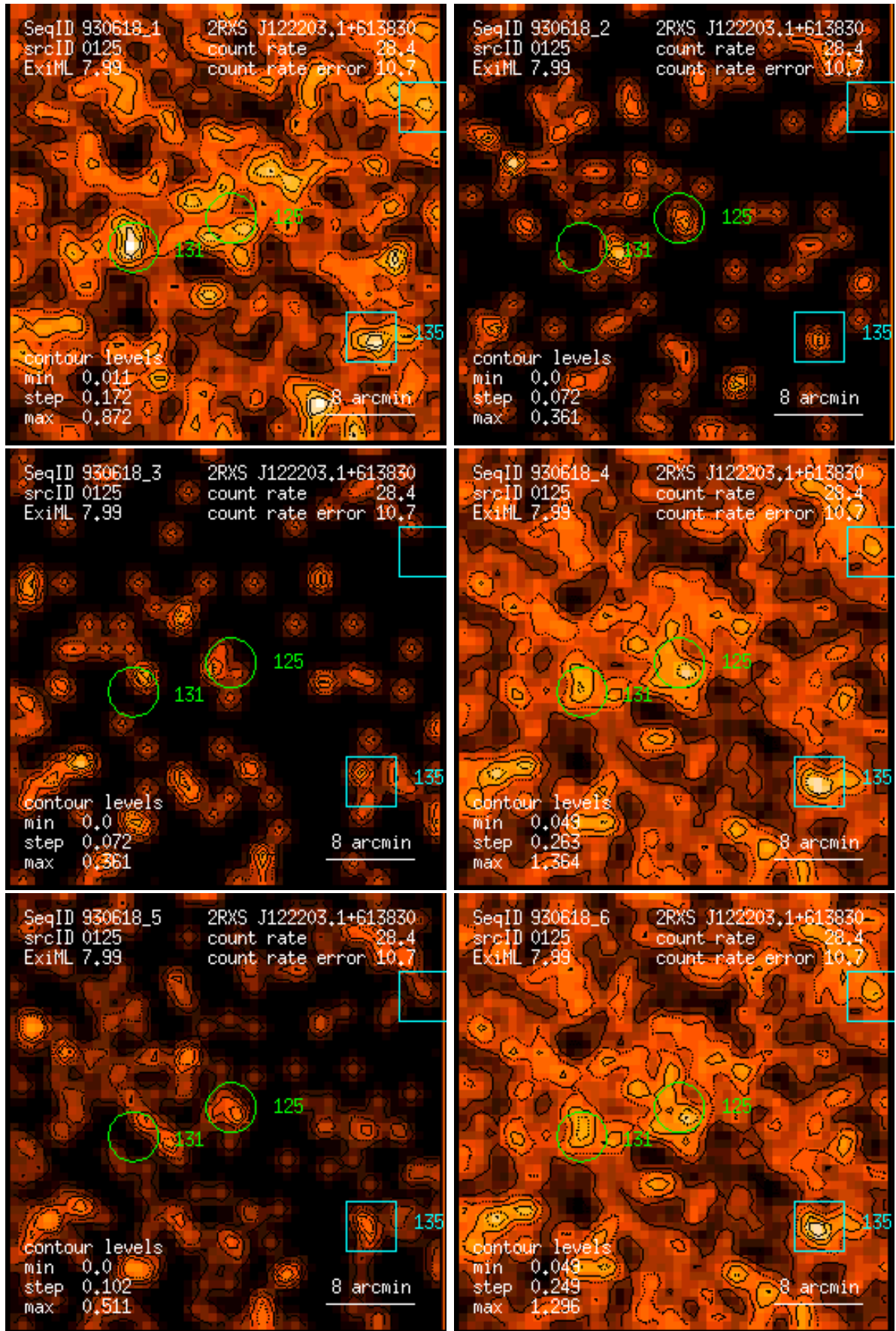
Figure 125: RASS 930618: detection 0125: band rate images, Gaussian filter: (1) PSPC channels 11 – 41, (2) 52 – 90, (3) 91 – 201, (4) 11 – 235, (5) 52 – 201, (6) 11 – 201. Broad band rates in counts/ks. Band rate contour levels in counts/ks/arcmin 2 .
