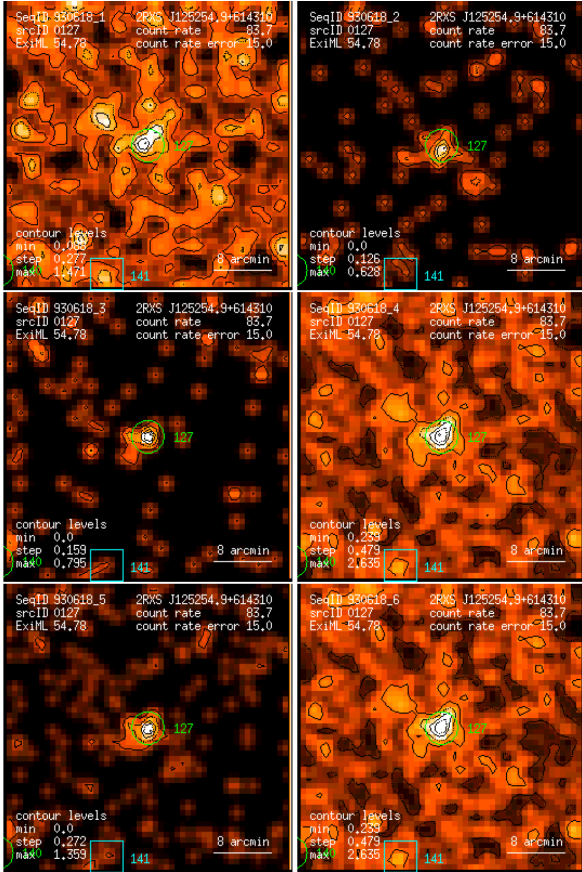
Figure 127: RASS 930618: detection 0127: band rate images, Gaussian filter: (1) PSPC channels 11 – 41, (2) 52 – 90, (3) 91 – 201, (4) 11 – 235, (5) 52 – 201, (6) 11 – 201. Broad band rates in counts/ks. Band rate contour levels in counts/ks/arcmin 2 .
