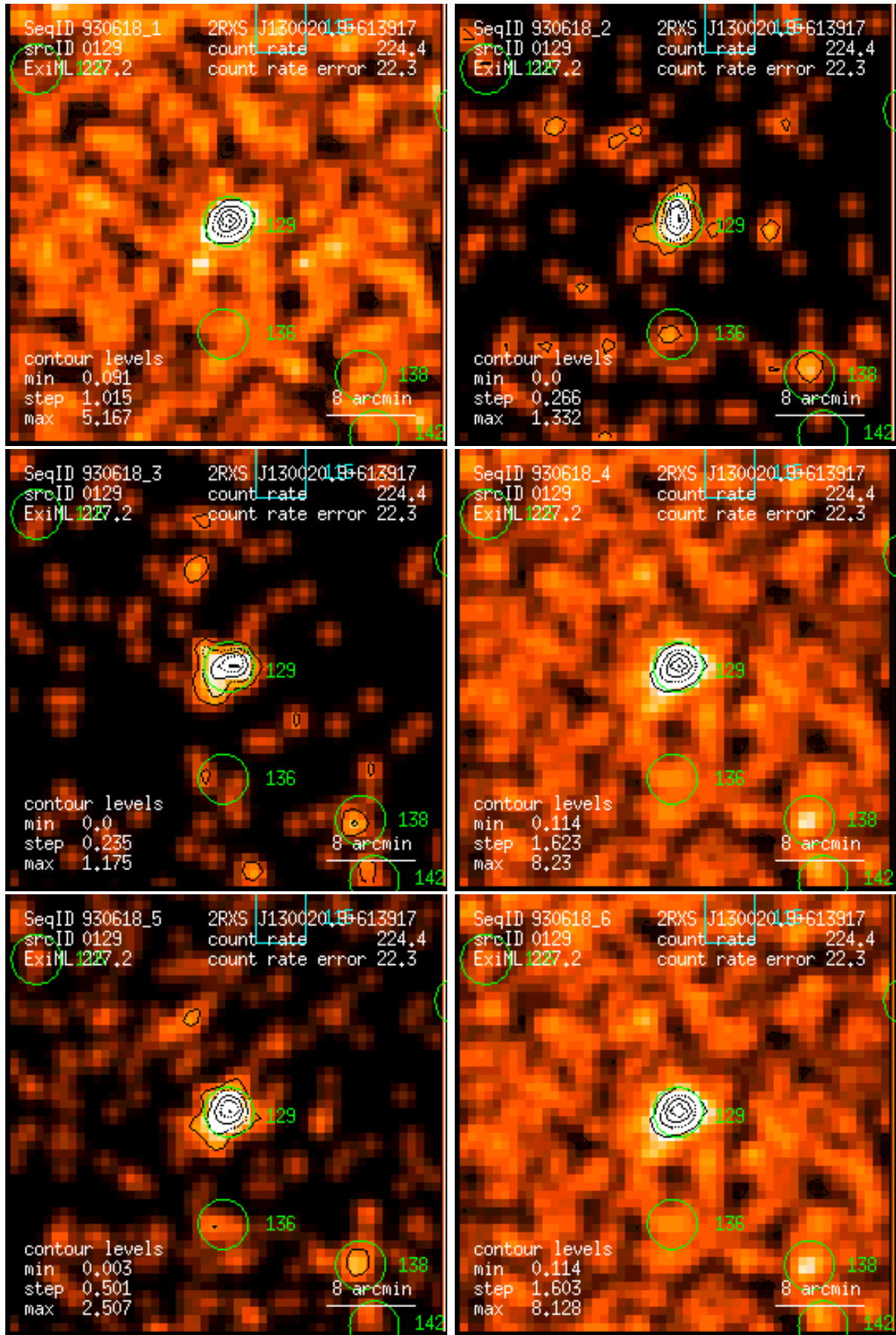
Figure 129: RASS 930618: detection 0129: band rate images, Gaussian filter: (1) PSPC channels 11 – 41, (2) 52 – 90, (3) 91 – 201, (4) 11 – 235, (5) 52 – 201, (6) 11 – 201. Broad band rates in counts/ks. Band rate contour levels in counts/ks/arcmin 2 .
