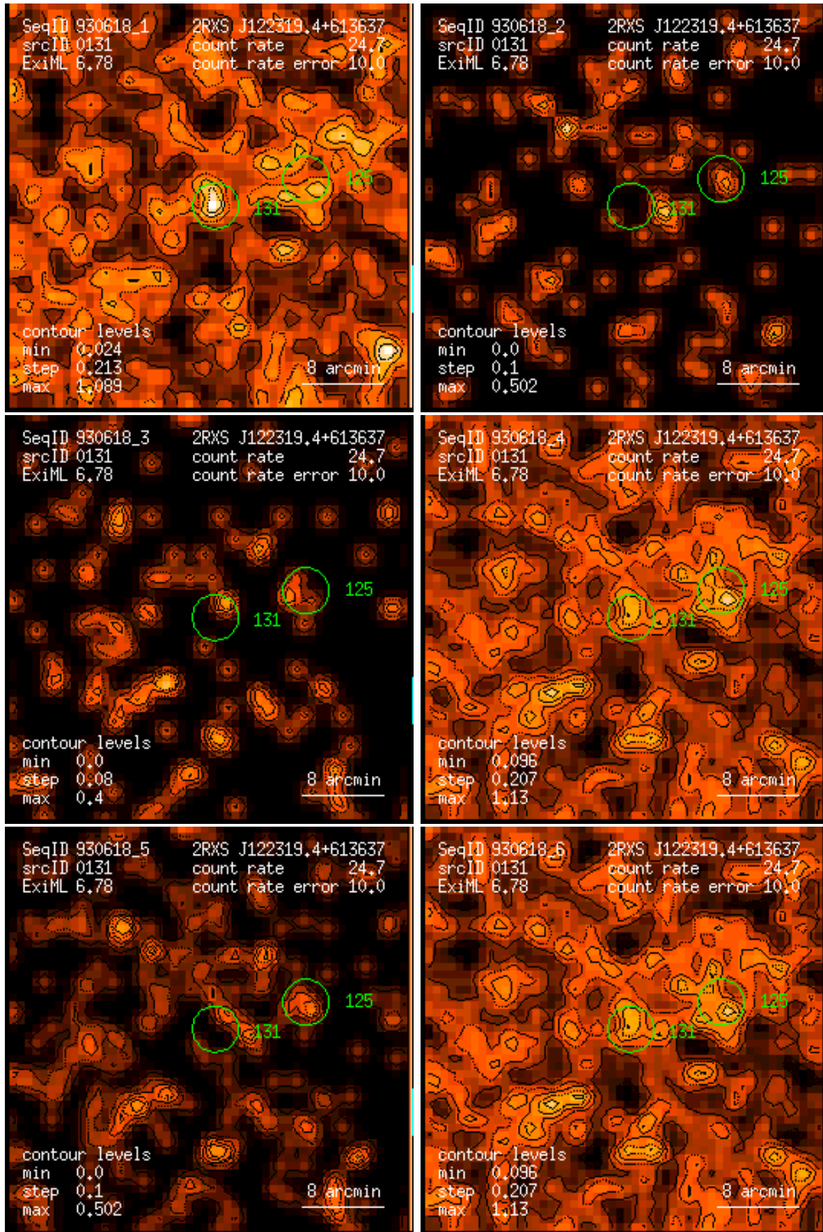
Figure 131: RASS 930618: detection 0131: band rate images, Gaussian filter: (1) PSPC channels 11 – 41, (2) 52 – 90, (3) 91 – 201, (4) 11 – 235, (5) 52 – 201, (6) 11 – 201. Broad band rates in counts/ks. Band rate contour levels in counts/ks/arcmin 2 .
