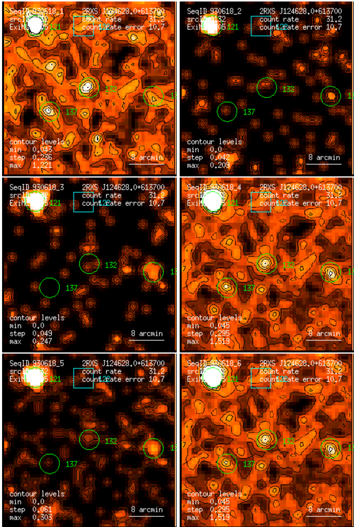
Figure 132: RASS 930618: detection 0132: band rate images, Gaussian filter: (1) PSPC channels 11 – 41, (2) 52 – 90, (3) 91 – 201, (4) 11 – 235, (5) 52 – 201, (6) 11 – 201. Broad band rates in counts/ks. Band rate contour levels in counts/ks/arcmin 2 .
