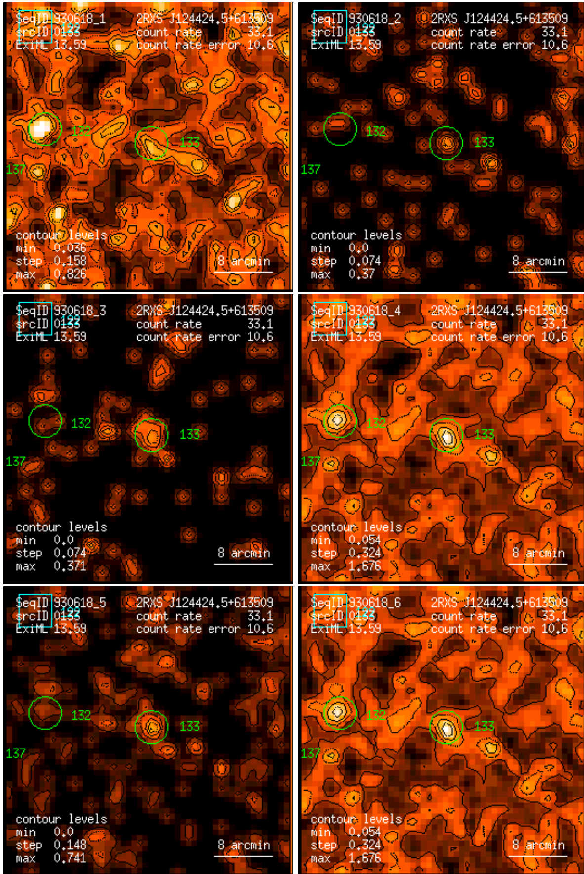
Figure 133: RASS 930618: detection 0133: band rate images, Gaussian filter: (1) PSPC channels 11 – 41, (2) 52 – 90, (3) 91 – 201, (4) 11 – 235, (5) 52 – 201, (6) 11 – 201. Broad band rates in counts/ks. Band rate contour levels in counts/ks/arcmin 2 .
