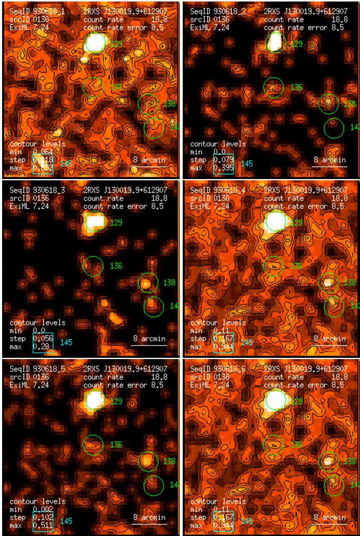
Figure 136: RASS 930618: detection 0136: band rate images, Gaussian filter: (1) PSPC channels 11 – 41, (2) 52 – 90, (3) 91 – 201, (4) 11 – 235, (5) 52 – 201, (6) 11 – 201. Broad band rates in counts/ks. Band rate contour levels in counts/ks/arcmin 2 .
