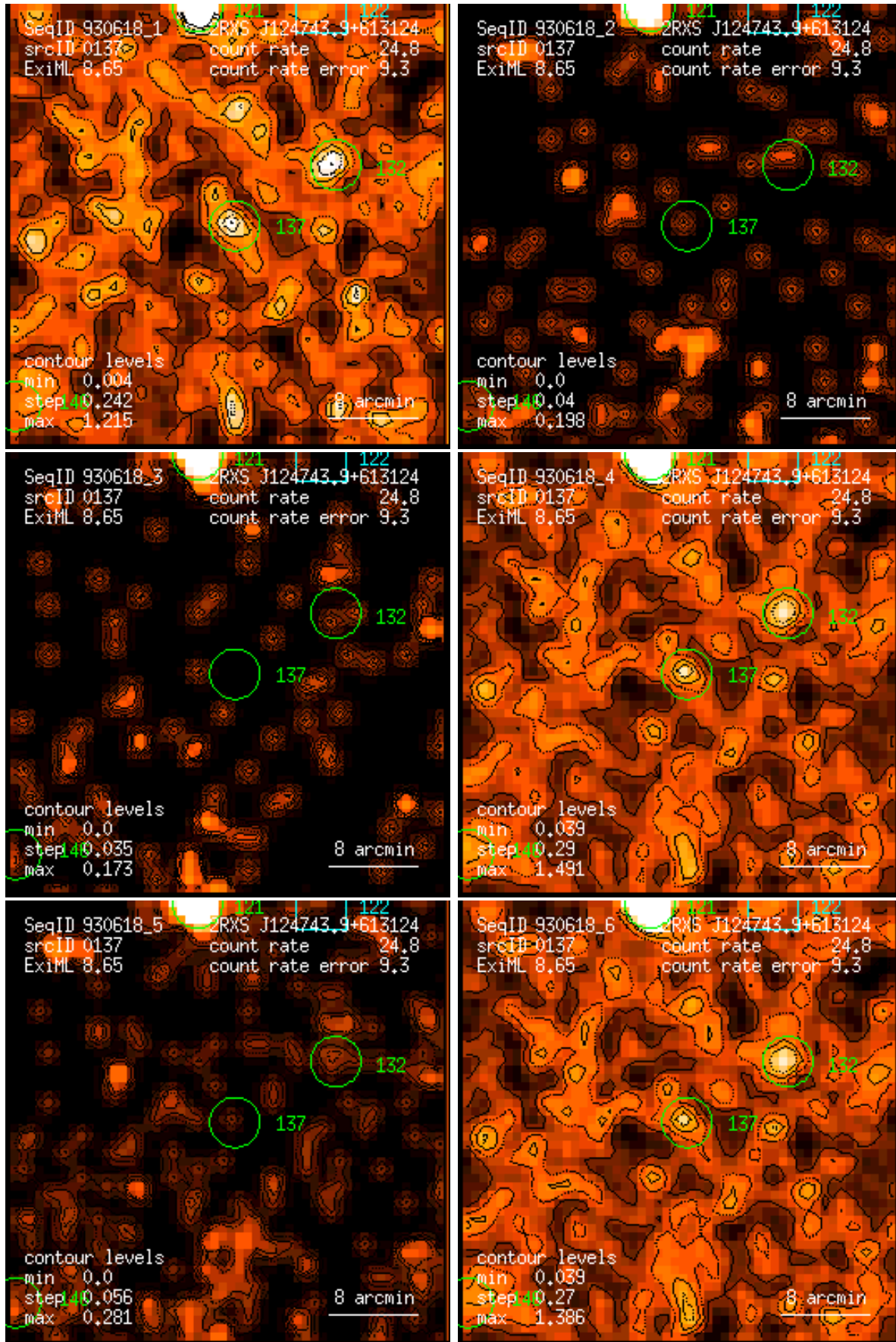
Figure 137: RASS 930618: detection 0137: band rate images, Gaussian filter: (1) PSPC channels 11 – 41, (2) 52 – 90, (3) 91 – 201, (4) 11 – 235, (5) 52 – 201, (6) 11 – 201. Broad band rates in counts/ks. Band rate contour levels in counts/ks/arcmin 2 .
