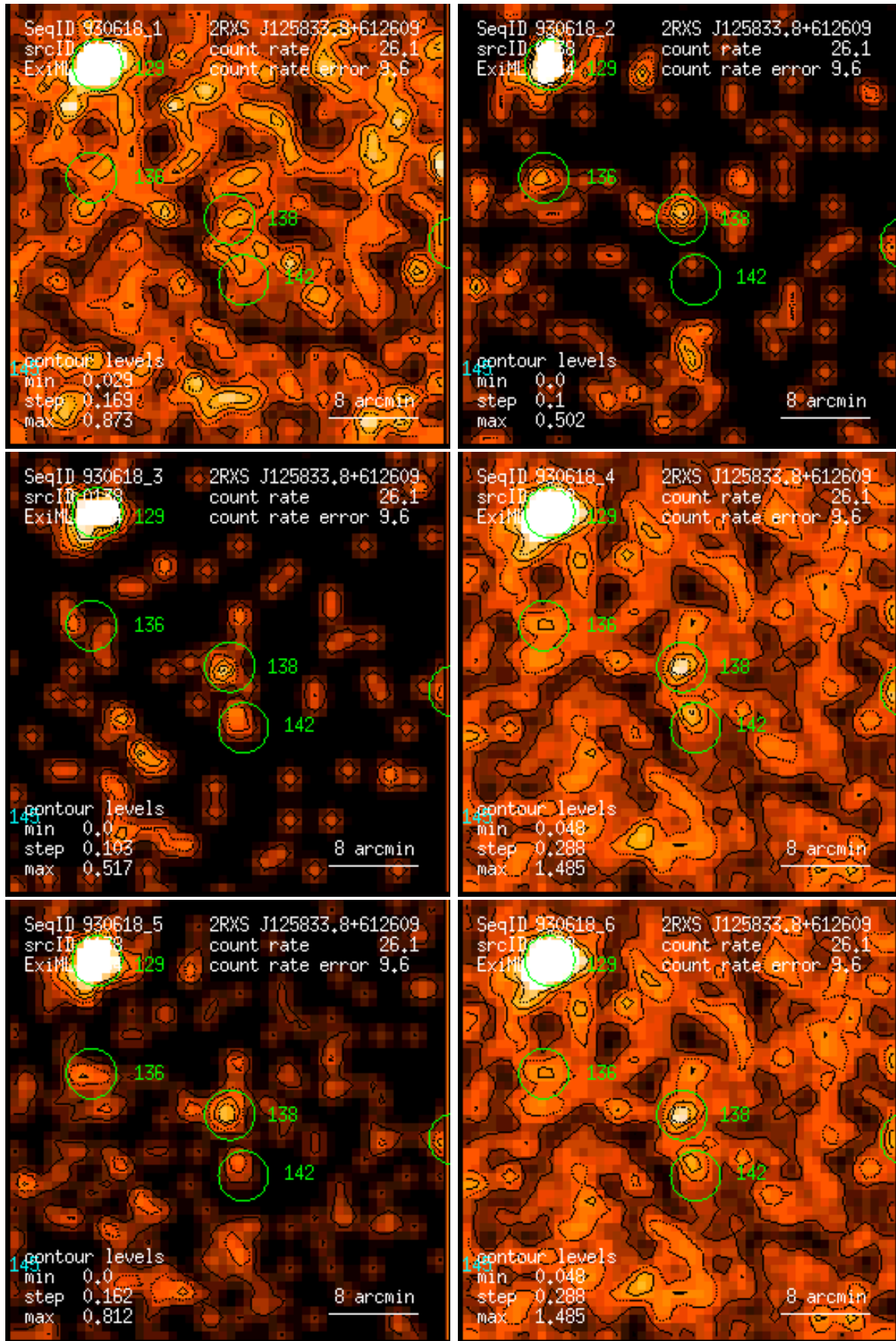
Figure 138: RASS 930618: detection 0138: band rate images, Gaussian filter: (1) PSPC channels 11 – 41, (2) 52 – 90, (3) 91 – 201, (4) 11 – 235, (5) 52 – 201, (6) 11 – 201. Broad band rates in counts/ks. Band rate contour levels in counts/ks/arcmin 2 .
