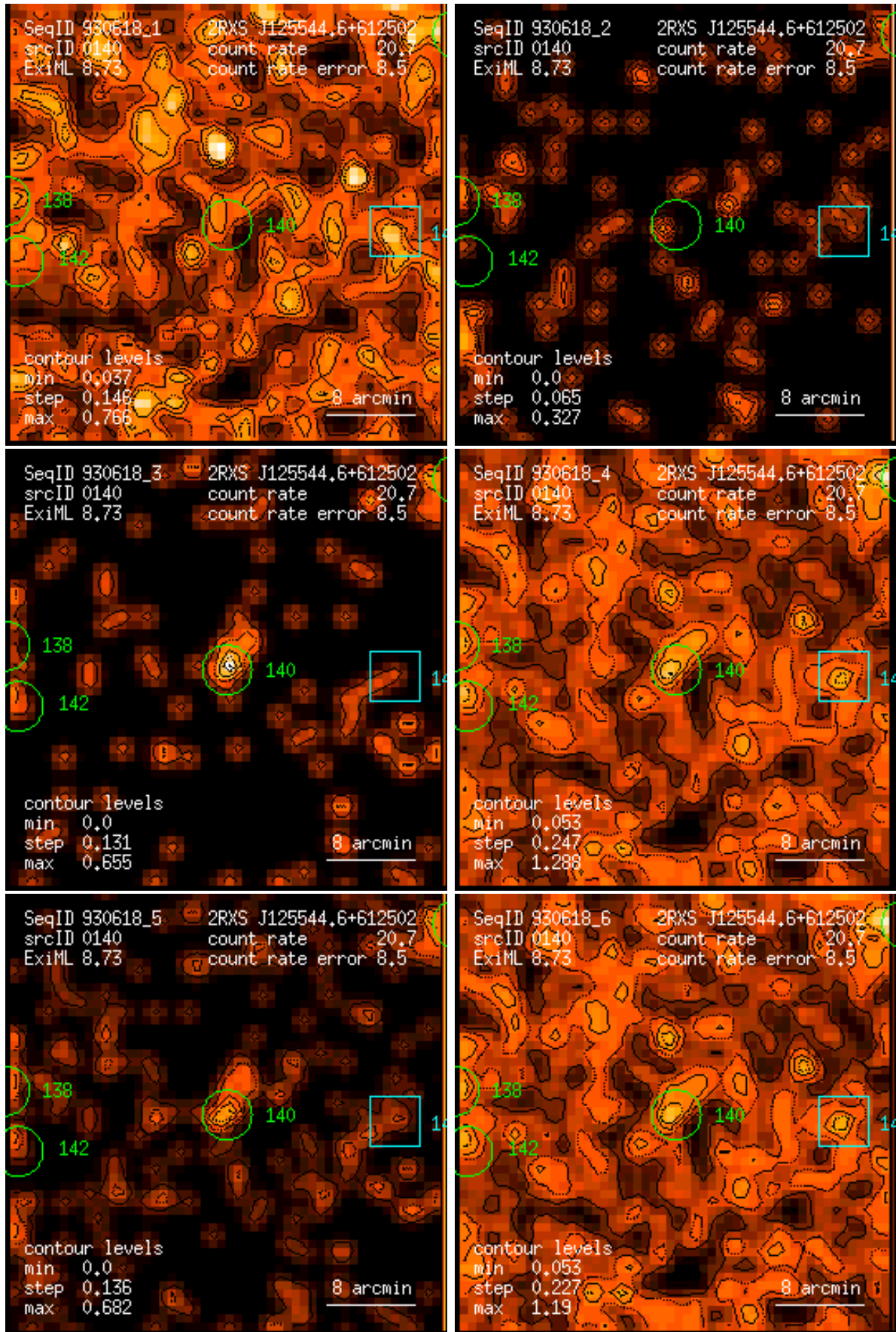
Figure 140: RASS 930618: detection 0140: band rate images, Gaussian filter: (1) PSPC channels 11 – 41, (2) 52 – 90, (3) 91 – 201, (4) 11 – 235, (5) 52 – 201, (6) 11 – 201. Broad band rates in counts/ks. Band rate contour levels in counts/ks/arcmin 2 .
