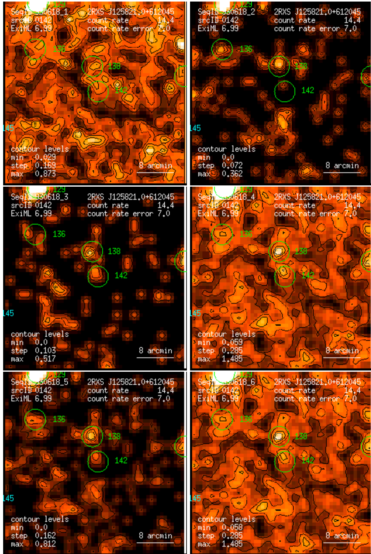
Figure 142: RASS 930618: detection 0142: band rate images, Gaussian filter: (1) PSPC channels 11 – 41, (2) 52 – 90, (3) 91 – 201, (4) 11 – 235, (5) 52 – 201, (6) 11 – 201. Broad band rates in counts/ks. Band rate contour levels in counts/ks/arcmin 2 .
