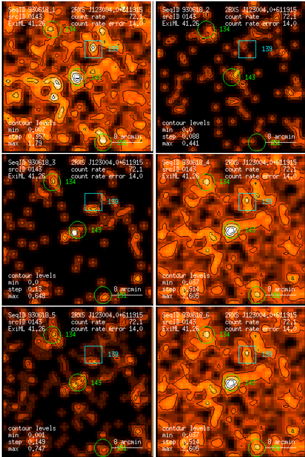
Figure 143: RASS 930618: detection 0143: band rate images, Gaussian filter: (1) PSPC channels 11 – 41, (2) 52 – 90, (3) 91 – 201, (4) 11 – 235, (5) 52 – 201, (6) 11 – 201. Broad band rates in counts/ks. Band rate contour levels in counts/ks/arcmin 2 .
