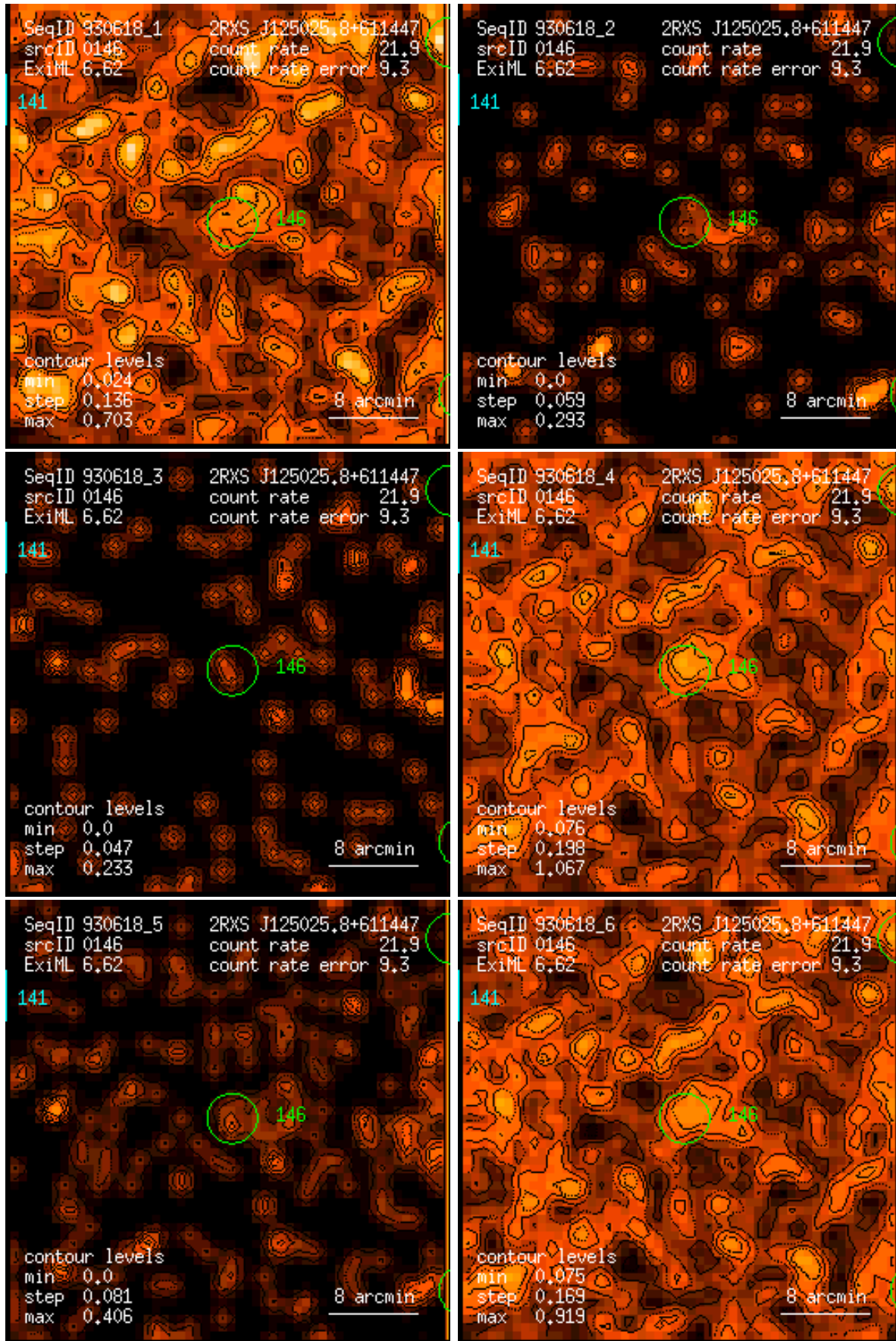
Figure 146: RASS 930618: detection 0146: band rate images, Gaussian filter: (1) PSPC channels 11 – 41, (2) 52 – 90, (3) 91 – 201, (4) 11 – 235, (5) 52 – 201, (6) 11 – 201. Broad band rates in counts/ks. Band rate contour levels in counts/ks/arcmin 2 .
