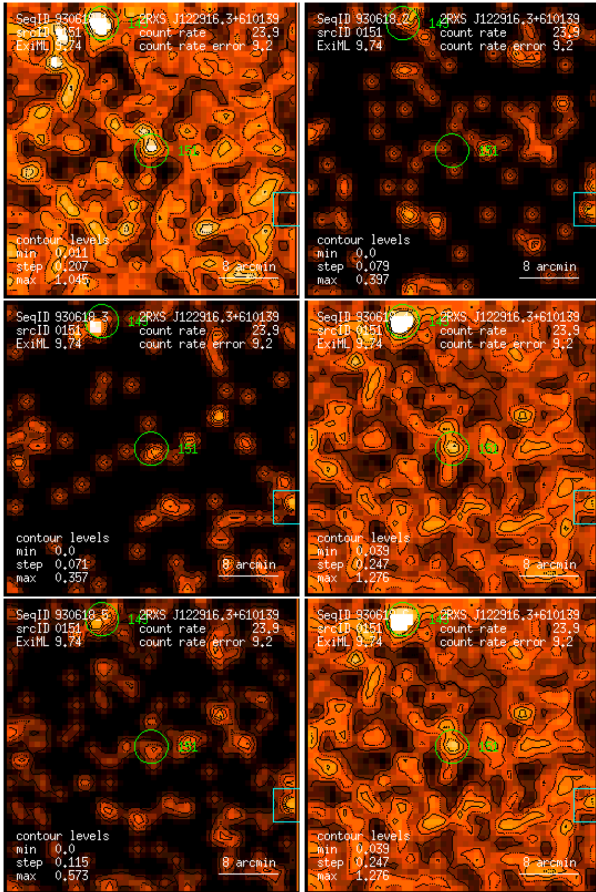
Figure 151: RASS 930618: detection 0151: band rate images, Gaussian filter: (1) PSPC channels 11 – 41, (2) 52 – 90, (3) 91 – 201, (4) 11 – 235, (5) 52 – 201, (6) 11 – 201. Broad band rates in counts/ks. Band rate contour levels in counts/ks/arcmin 2 .
