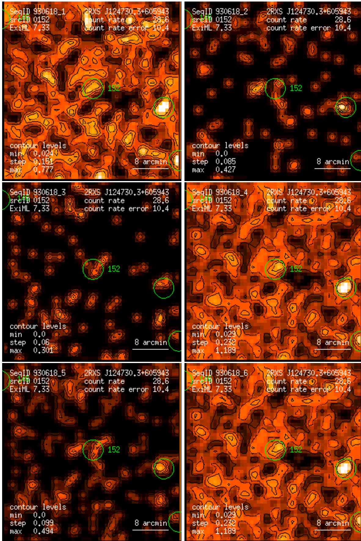
Figure 152: RASS 930618: detection 0152: band rate images, Gaussian filter: (1) PSPC channels 11 – 41, (2) 52 – 90, (3) 91 – 201, (4) 11 – 235, (5) 52 – 201, (6) 11 – 201. Broad band rates in counts/ks. Band rate contour levels in counts/ks/arcmin 2 .
