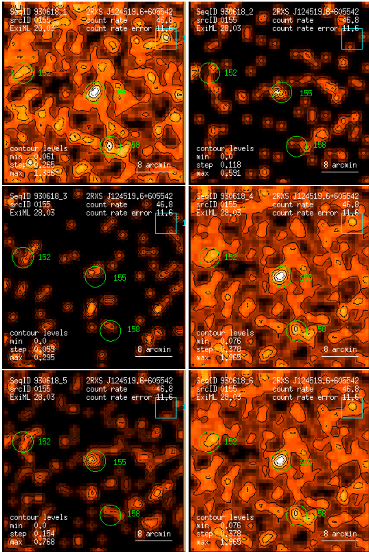
Figure 155: RASS 930618: detection 0155: band rate images, Gaussian filter: (1) PSPC channels 11 – 41, (2) 52 – 90, (3) 91 – 201, (4) 11 – 235, (5) 52 – 201, (6) 11 – 201. Broad band rates in counts/ks. Band rate contour levels in counts/ks/arcmin 2 .
