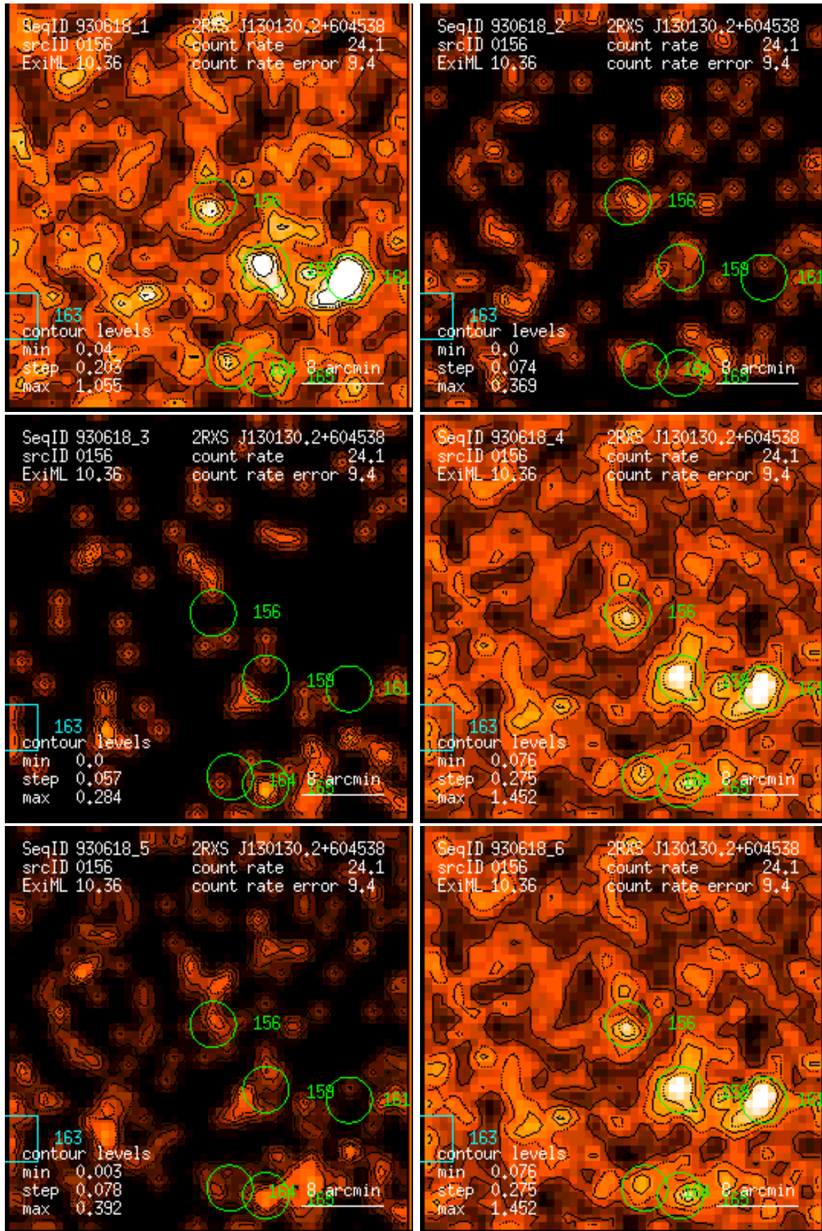
Figure 156: RASS 930618: detection 0156: band rate images, Gaussian filter: (1) PSPC channels 11 – 41, (2) 52 – 90, (3) 91 – 201, (4) 11 – 235, (5) 52 – 201, (6) 11 – 201. Broad band rates in counts/ks. Band rate contour levels in counts/ks/arcmin 2 .
