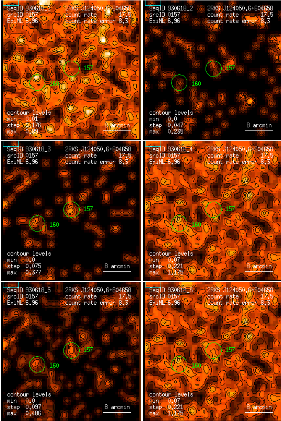
Figure 157: RASS 930618: detection 0157: band rate images, Gaussian filter: (1) PSPC channels 11 – 41, (2) 52 – 90, (3) 91 – 201, (4) 11 – 235, (5) 52 – 201, (6) 11 – 201. Broad band rates in counts/ks. Band rate contour levels in counts/ks/arcmin 2 .
