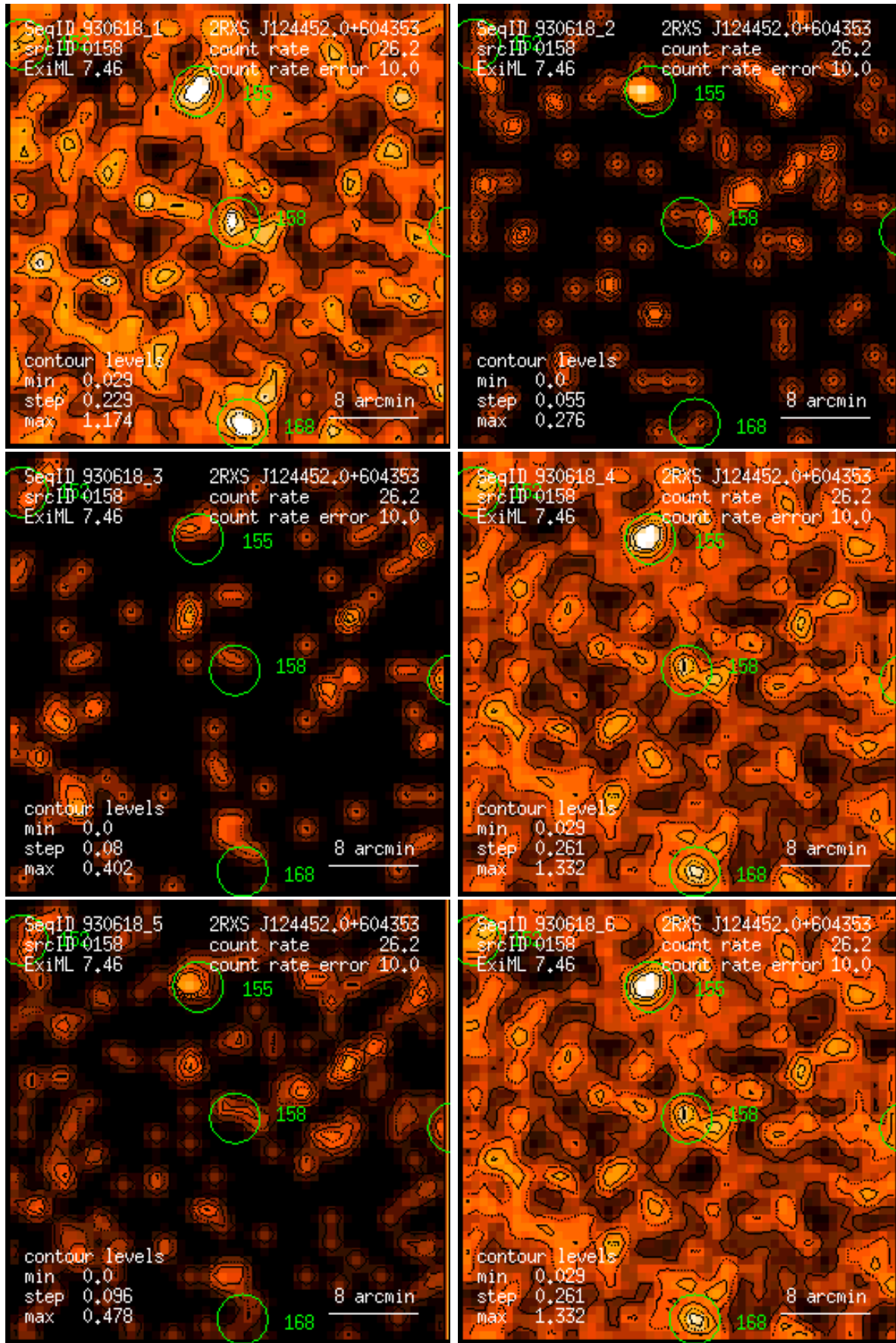
Figure 158: RASS 930618: detection 0158: band rate images, Gaussian filter: (1) PSPC channels 11 – 41, (2) 52 – 90, (3) 91 – 201, (4) 11 – 235, (5) 52 – 201, (6) 11 – 201. Broad band rates in counts/ks. Band rate contour levels in counts/ks/arcmin 2 .
