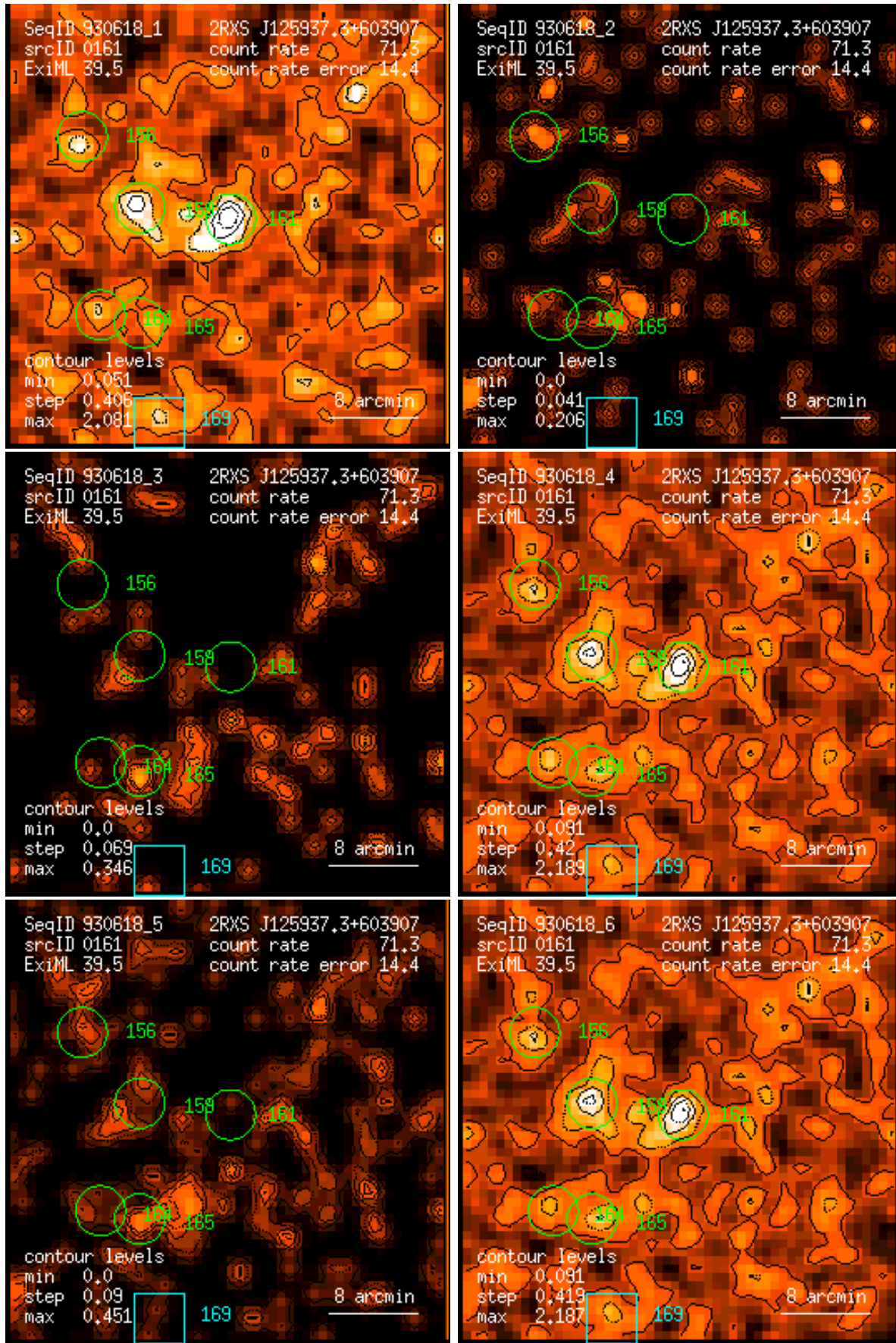
Figure 161: RASS 930618: detection 0161: band rate images, Gaussian filter: (1) PSPC channels 11 – 41, (2) 52 – 90, (3) 91 – 201, (4) 11 – 235, (5) 52 – 201, (6) 11 – 201. Broad band rates in counts/ks. Band rate contour levels in counts/ks/arcmin 2 .
