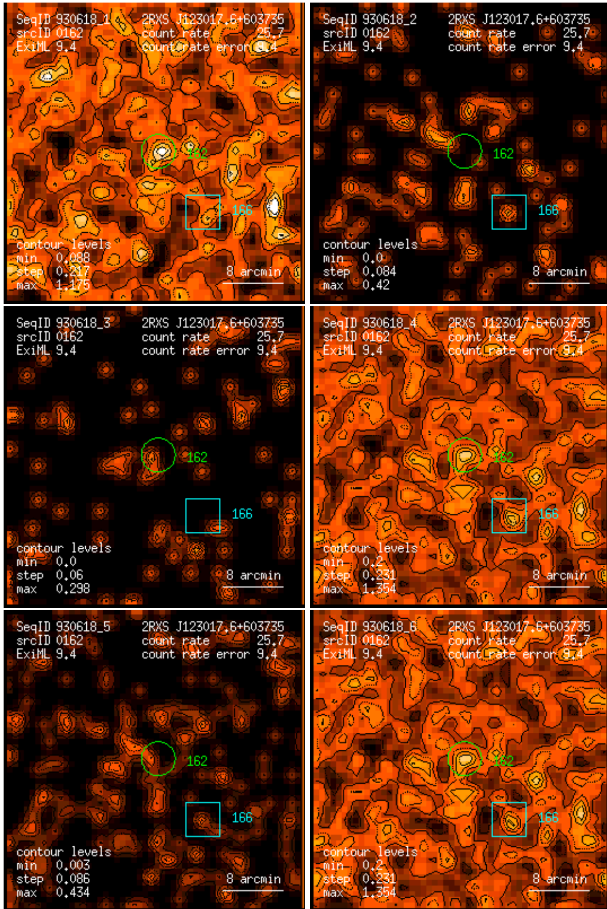
Figure 162: RASS 930618: detection 0162: band rate images, Gaussian filter: (1) PSPC channels 11 – 41, (2) 52 – 90, (3) 91 – 201, (4) 11 – 235, (5) 52 – 201, (6) 11 – 201. Broad band rates in counts/ks. Band rate contour levels in counts/ks/arcmin 2 .
