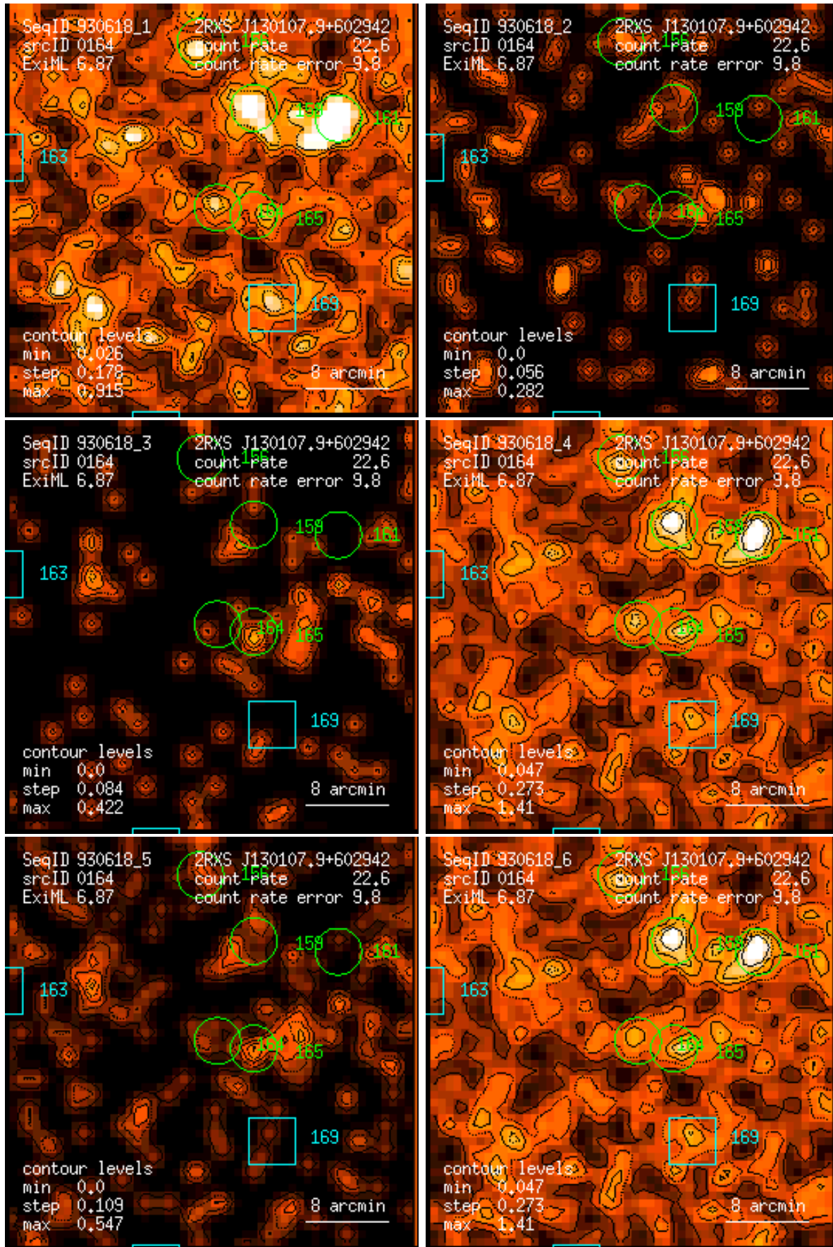
Figure 164: RASS 930618: detection 0164: band rate images, Gaussian filter: (1) PSPC channels 11 – 41, (2) 52 – 90, (3) 91 – 201, (4) 11 – 235, (5) 52 – 201, (6) 11 – 201. Broad band rates in counts/ks. Band rate contour levels in counts/ks/arcmin 2 .
