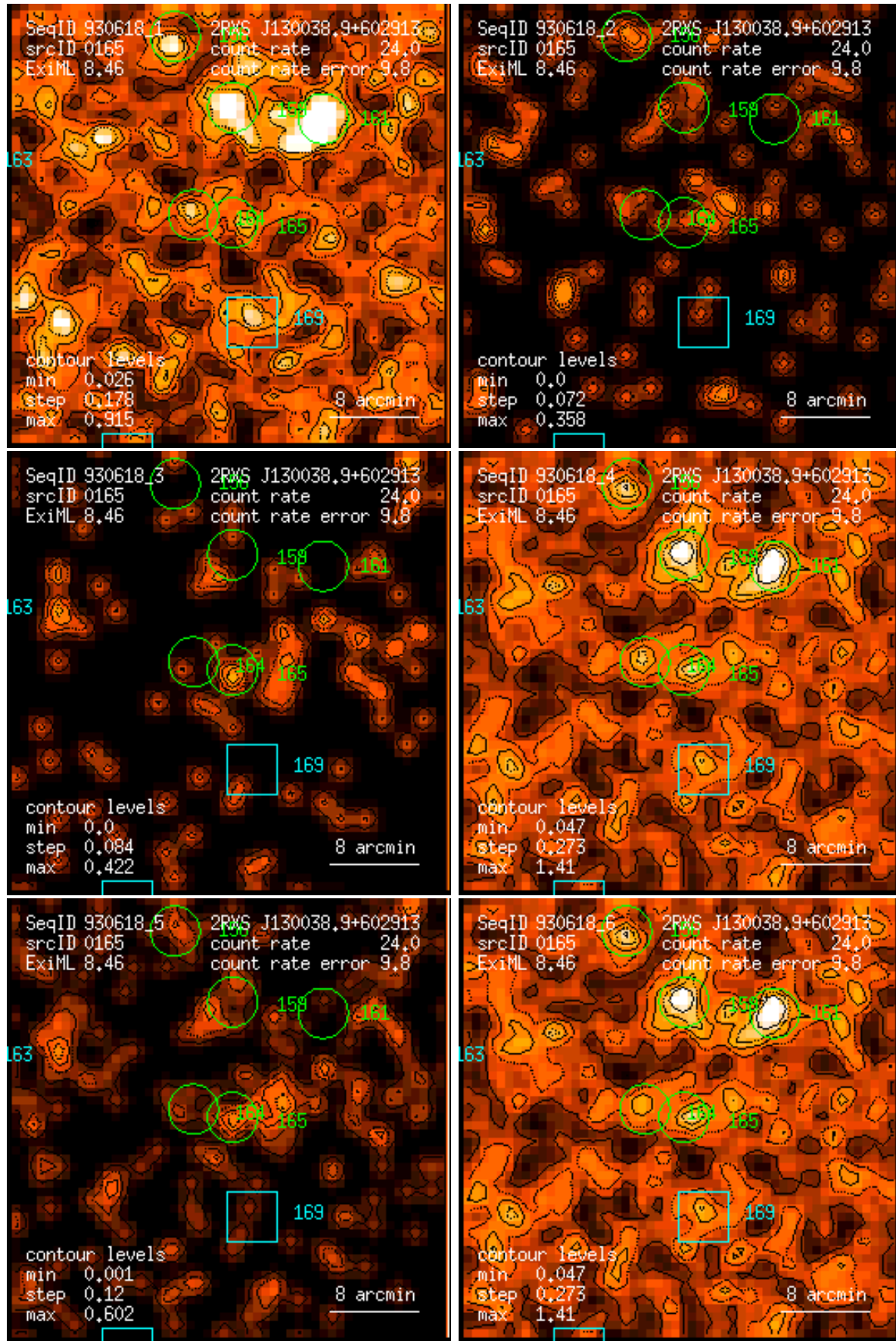
Figure 165: RASS 930618: detection 0165: band rate images, Gaussian filter: (1) PSPC channels 11 – 41, (2) 52 – 90, (3) 91 – 201, (4) 11 – 235, (5) 52 – 201, (6) 11 – 201. Broad band rates in counts/ks. Band rate contour levels in counts/ks/arcmin 2 .
