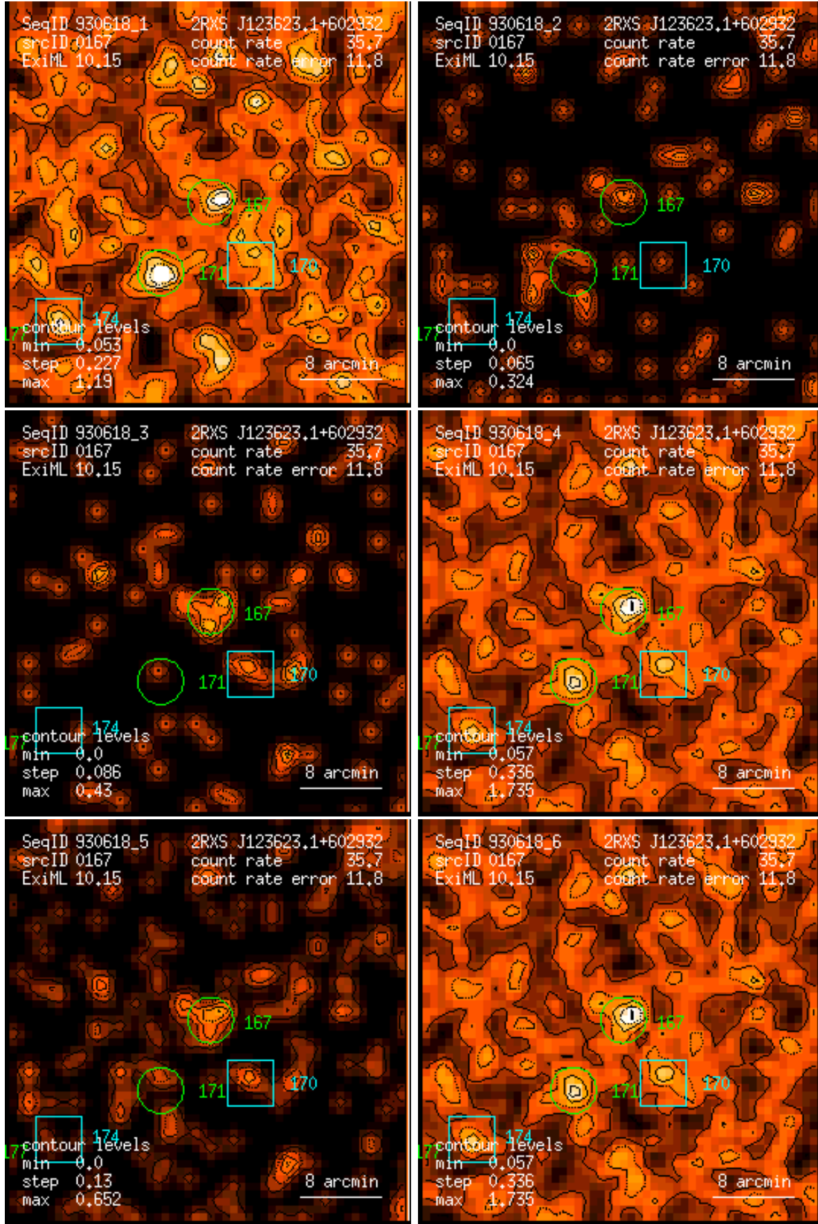
Figure 167: RASS 930618: detection 0167: band rate images, Gaussian filter: (1) PSPC channels 11 – 41, (2) 52 – 90, (3) 91 – 201, (4) 11 – 235, (5) 52 – 201, (6) 11 – 201. Broad band rates in counts/ks. Band rate contour levels in counts/ks/arcmin 2 .
