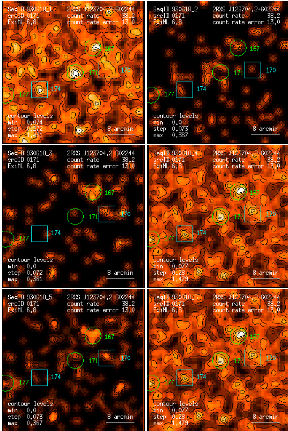
Figure 171: RASS 930618: detection 0171: band rate images, Gaussian filter: (1) PSPC channels 11 – 41, (2) 52 – 90, (3) 91 – 201, (4) 11 – 235, (5) 52 – 201, (6) 11 – 201. Broad band rates in counts/ks. Band rate contour levels in counts/ks/arcmin 2 .
