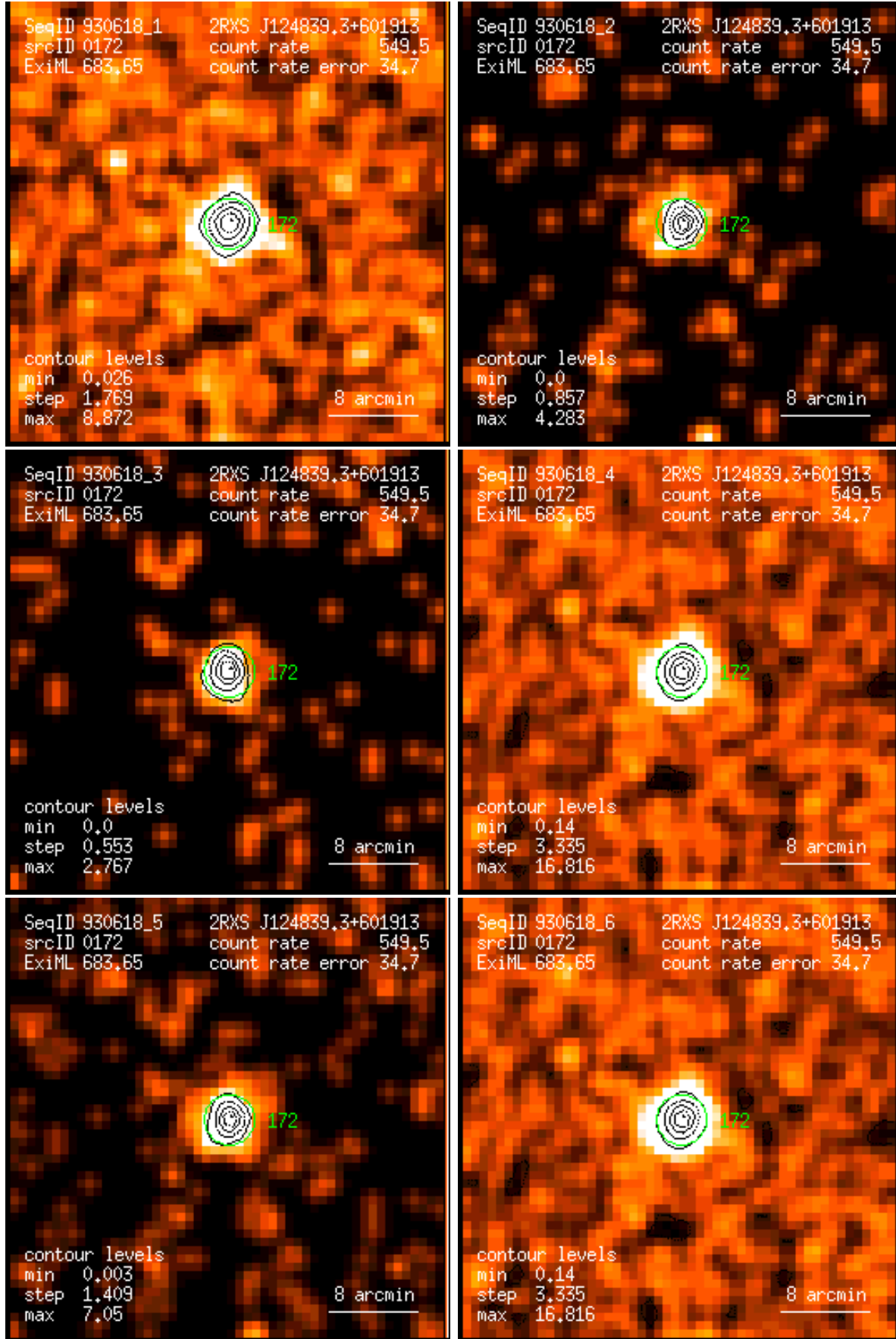
Figure 172: RASS 930618: detection 0172: band rate images, Gaussian filter: (1) PSPC channels 11 – 41, (2) 52 – 90, (3) 91 – 201, (4) 11 – 235, (5) 52 – 201, (6) 11 – 201. Broad band rates in counts/ks. Band rate contour levels in counts/ks/arcmin 2 .
