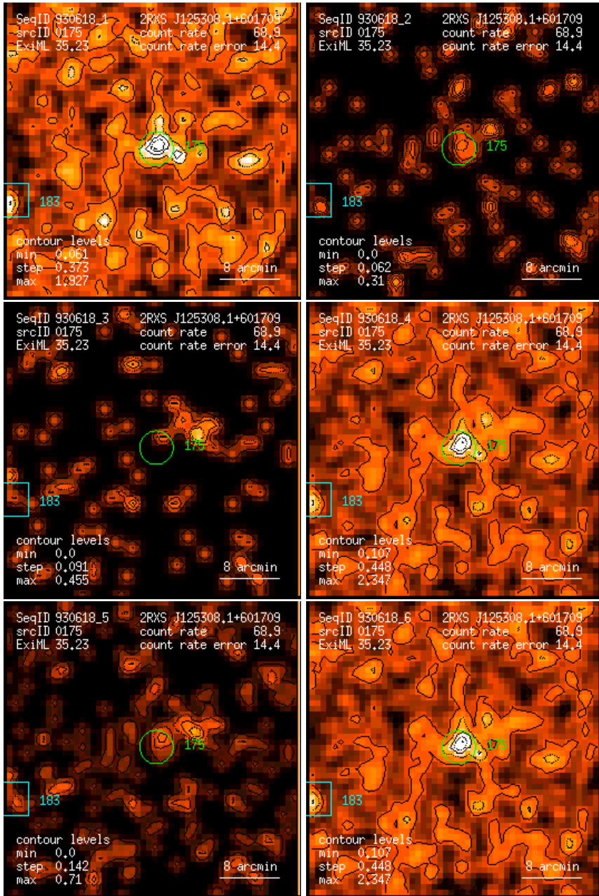
Figure 175: RASS 930618: detection 0175: band rate images, Gaussian filter: (1) PSPC channels 11 – 41, (2) 52 – 90, (3) 91 – 201, (4) 11 – 235, (5) 52 – 201, (6) 11 – 201. Broad band rates in counts/ks. Band rate contour levels in counts/ks/arcmin 2 .
