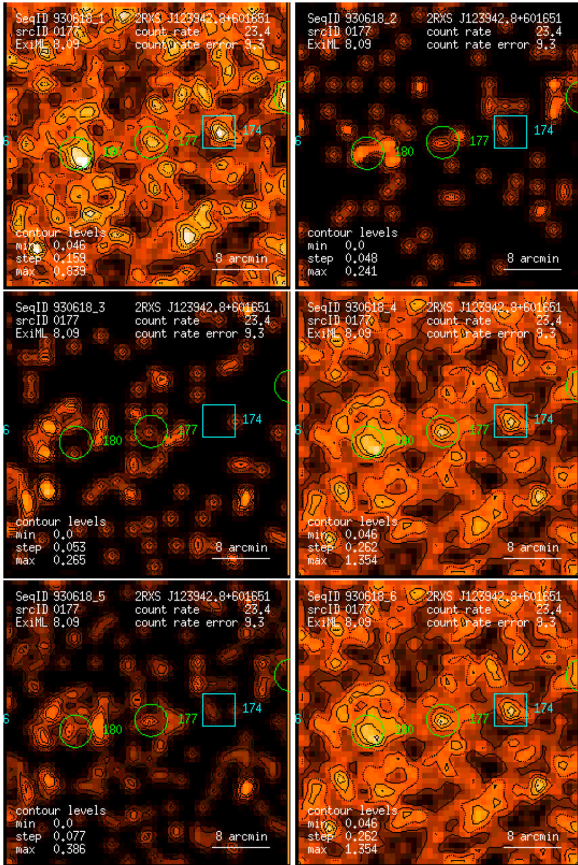
Figure 177: RASS 930618: detection 0177: band rate images, Gaussian filter: (1) PSPC channels 11 – 41, (2) 52 – 90, (3) 91 – 201, (4) 11 – 235, (5) 52 – 201, (6) 11 – 201. Broad band rates in counts/ks. Band rate contour levels in counts/ks/arcmin 2 .
