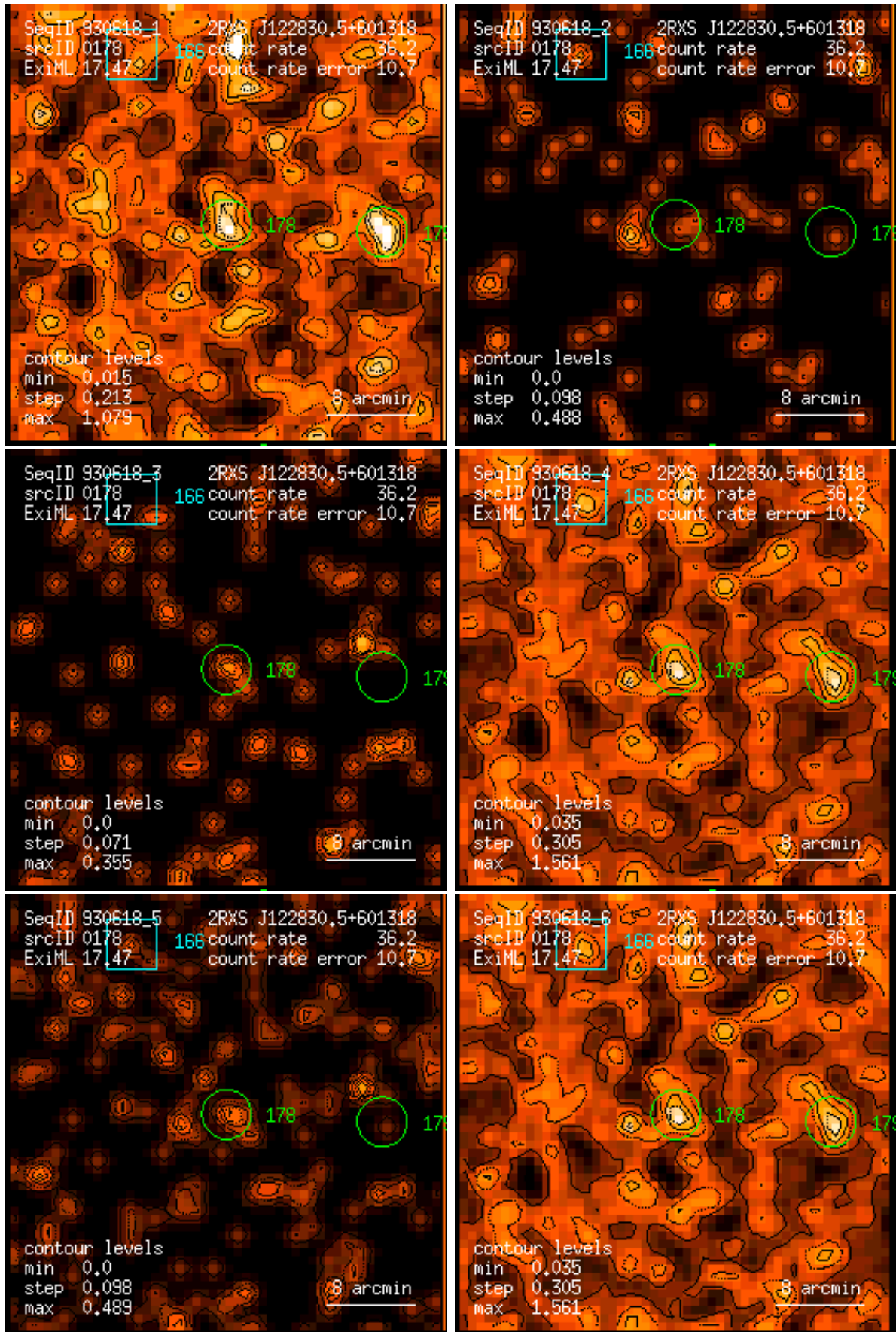
Figure 178: RASS 930618: detection 0178: band rate images, Gaussian filter: (1) PSPC channels 11 – 41, (2) 52 – 90, (3) 91 – 201, (4) 11 – 235, (5) 52 – 201, (6) 11 – 201. Broad band rates in counts/ks. Band rate contour levels in counts/ks/arcmin 2 .
