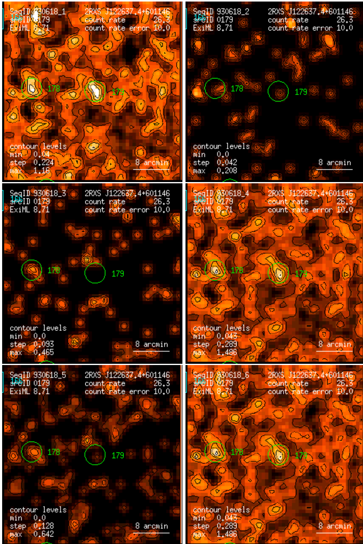
Figure 179: RASS 930618: detection 0179: band rate images, Gaussian filter: (1) PSPC channels 11 – 41, (2) 52 – 90, (3) 91 – 201, (4) 11 – 235, (5) 52 – 201, (6) 11 – 201. Broad band rates in counts/ks. Band rate contour levels in counts/ks/arcmin 2 .
