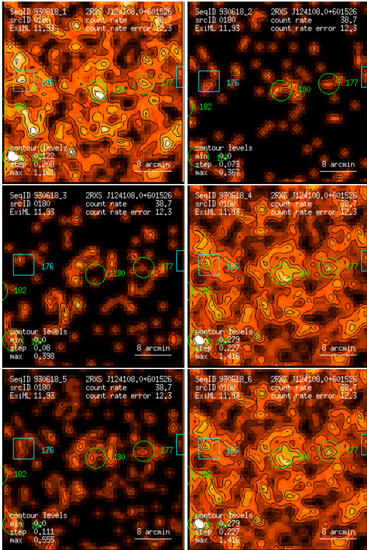
Figure 180: RASS 930618: detection 0180: band rate images, Gaussian filter: (1) PSPC channels 11 – 41, (2) 52 – 90, (3) 91 – 201, (4) 11 – 235, (5) 52 – 201, (6) 11 – 201. Broad band rates in counts/ks. Band rate contour levels in counts/ks/arcmin 2 .
