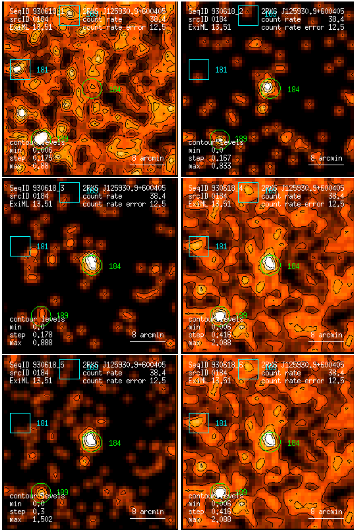
Figure 184: RASS 930618: detection 0184: band rate images, Gaussian filter: (1) PSPC channels 11 – 41, (2) 52 – 90, (3) 91 – 201, (4) 11 – 235, (5) 52 – 201, (6) 11 – 201. Broad band rates in counts/ks. Band rate contour levels in counts/ks/arcmin 2 .
