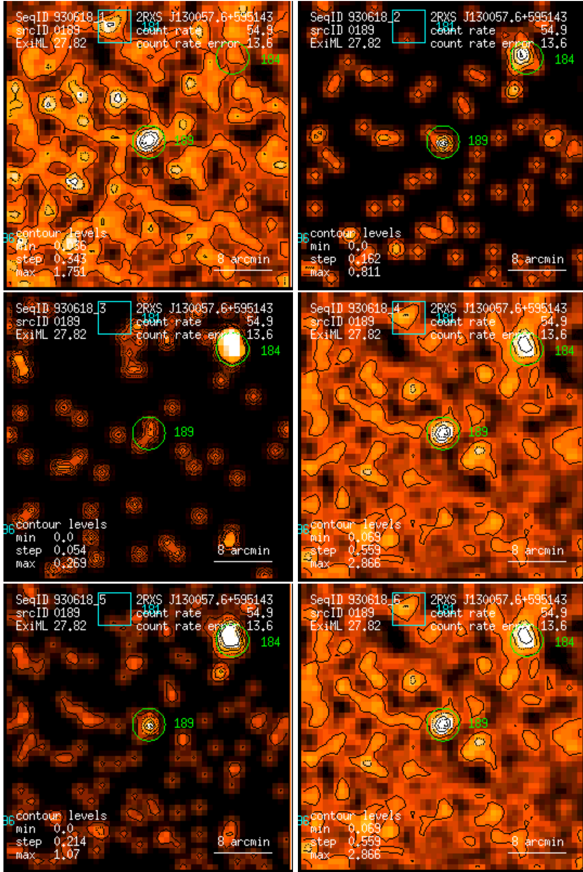
Figure 189: RASS 930618: detection 0189: band rate images, Gaussian filter: (1) PSPC channels 11 – 41, (2) 52 – 90, (3) 91 – 201, (4) 11 – 235, (5) 52 – 201, (6) 11 – 201. Broad band rates in counts/ks. Band rate contour levels in counts/ks/arcmin 2 .
