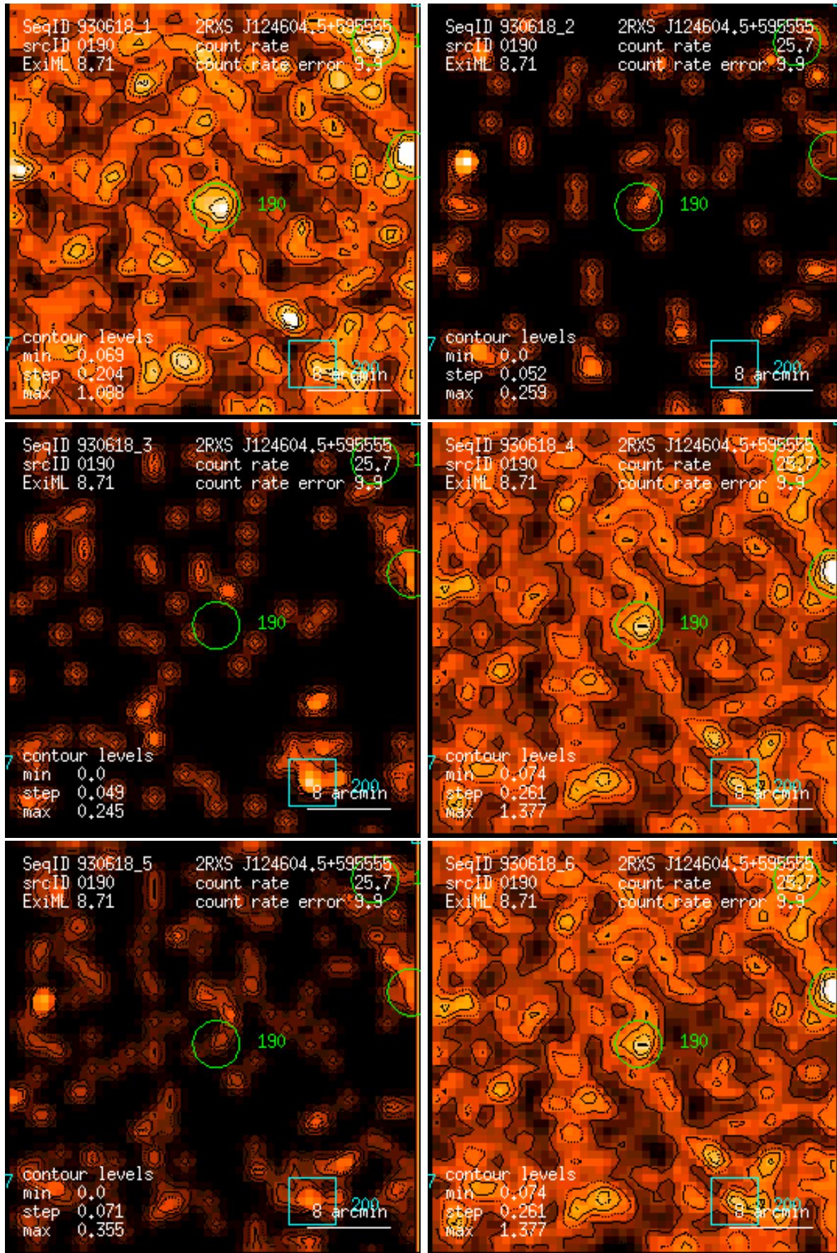
Figure 190: RASS 930618: detection 0190: band rate images, Gaussian filter: (1) PSPC channels 11 – 41, (2) 52 – 90, (3) 91 – 201, (4) 11 – 235, (5) 52 – 201, (6) 11 – 201. Broad band rates in counts/ks. Band rate contour levels in counts/ks/arcmin 2 .
