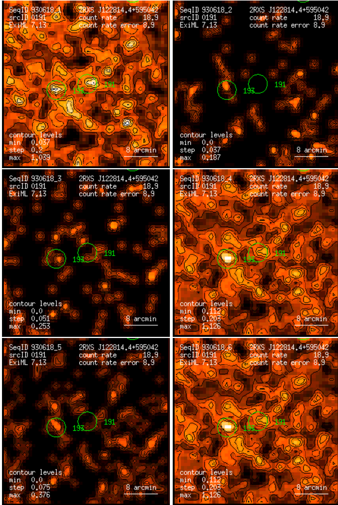
Figure 191: RASS 930618: detection 0191: band rate images, Gaussian filter: (1) PSPC channels 11 – 41, (2) 52 – 90, (3) 91 – 201, (4) 11 – 235, (5) 52 – 201, (6) 11 – 201. Broad band rates in counts/ks. Band rate contour levels in counts/ks/arcmin 2 .
