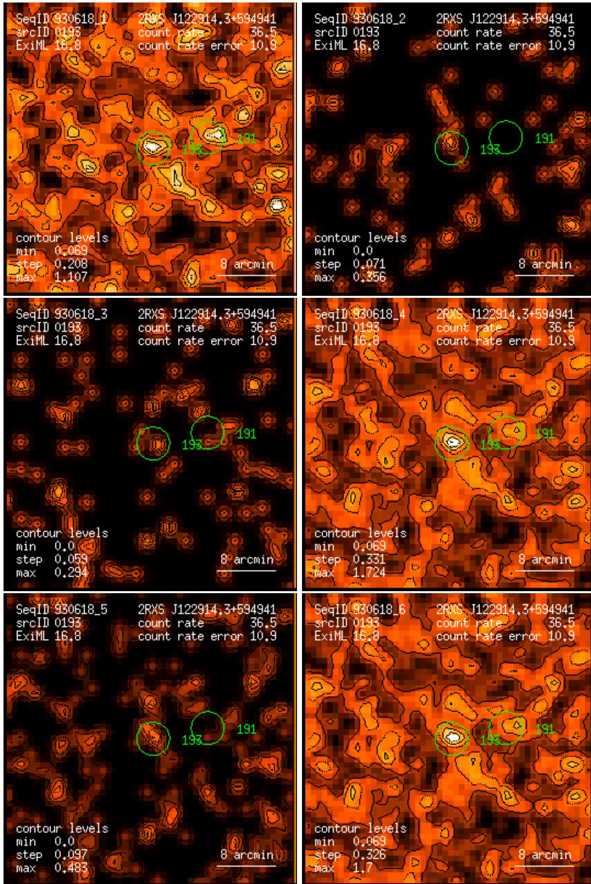
Figure 193: RASS 930618: detection 0193: band rate images, Gaussian filter: (1) PSPC channels 11 – 41, (2) 52 – 90, (3) 91 – 201, (4) 11 – 235, (5) 52 – 201, (6) 11 – 201. Broad band rates in counts/ks. Band rate contour levels in counts/ks/arcmin 2 .
