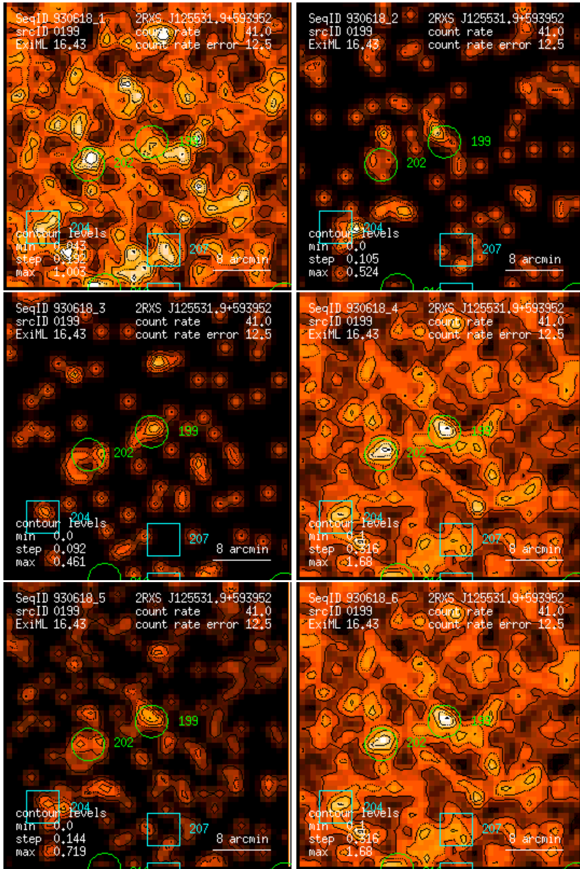
Figure 199: RASS 930618: detection 0199: band rate images, Gaussian filter: (1) PSPC channels 11 – 41, (2) 52 – 90, (3) 91 – 201, (4) 11 – 235, (5) 52 – 201, (6) 11 – 201. Broad band rates in counts/ks. Band rate contour levels in counts/ks/arcmin 2 .
