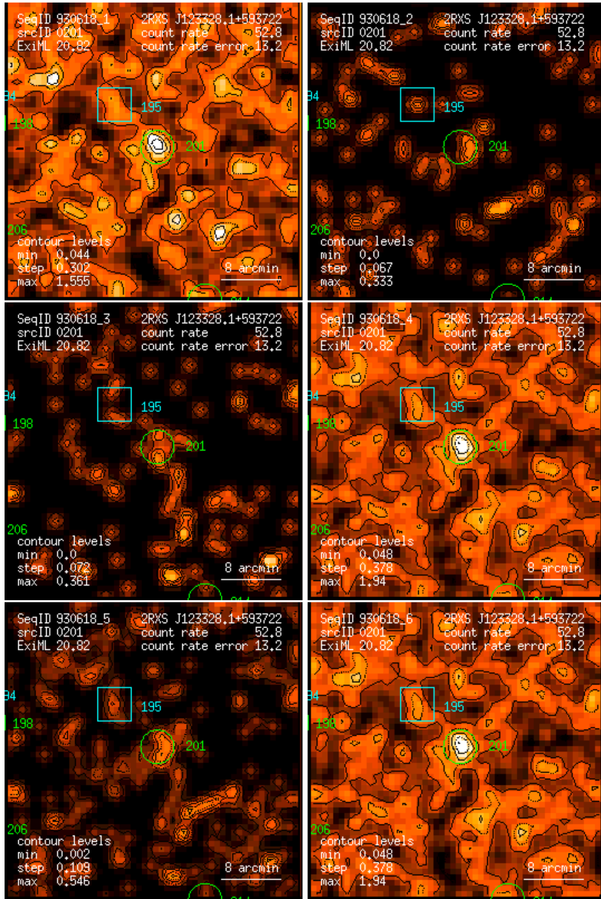
Figure 201: RASS 930618: detection 0201: band rate images, Gaussian filter: (1) PSPC channels 11 – 41, (2) 52 – 90, (3) 91 – 201, (4) 11 – 235, (5) 52 – 201, (6) 11 – 201. Broad band rates in counts/ks. Band rate contour levels in counts/ks/arcmin 2 .
