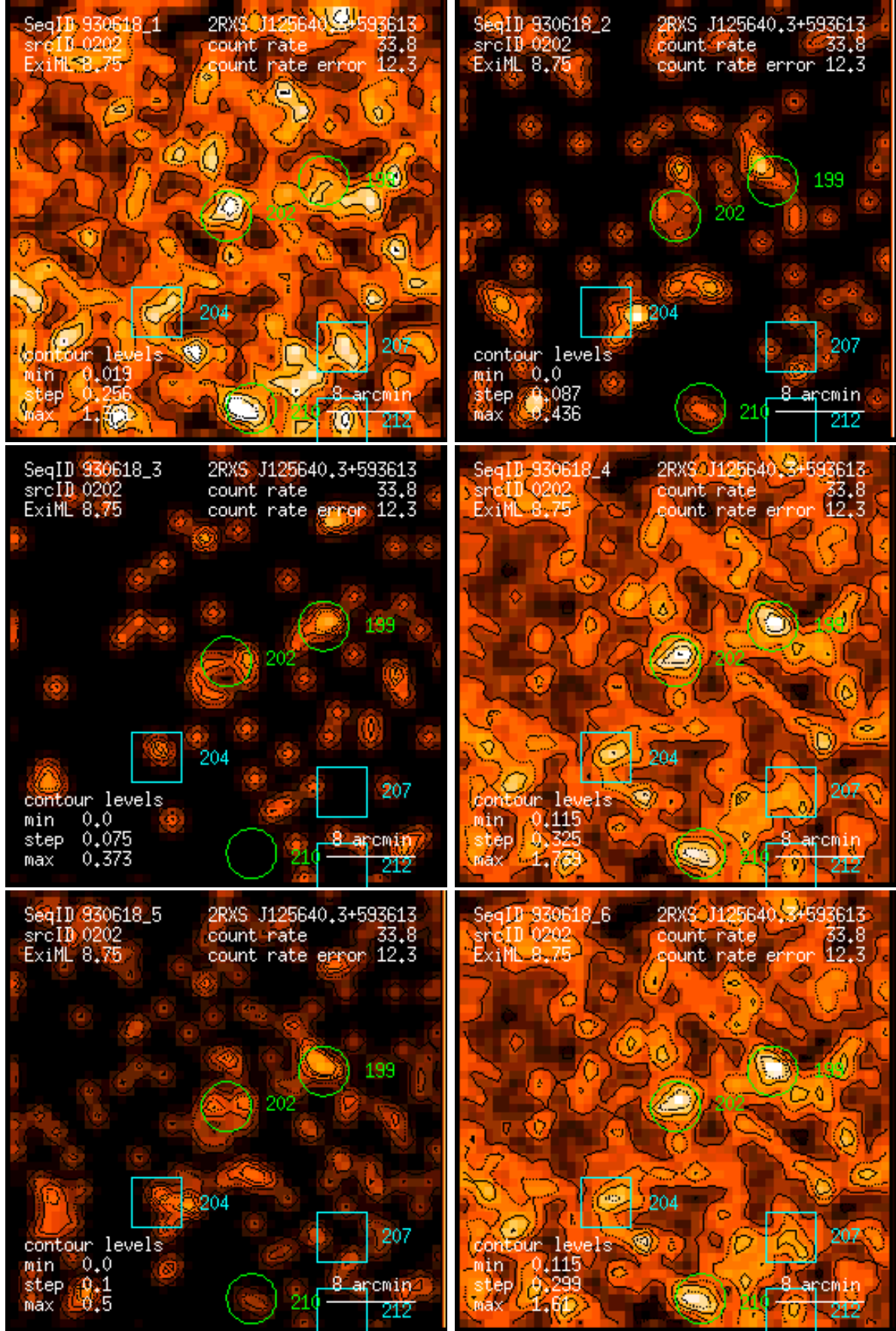
Figure 202: RASS 930618: detection 0202: band rate images, Gaussian filter: (1) PSPC channels 11 – 41, (2) 52 – 90, (3) 91 – 201, (4) 11 – 235, (5) 52 – 201, (6) 11 – 201. Broad band rates in counts/ks. Band rate contour levels in counts/ks/arcmin 2 .
