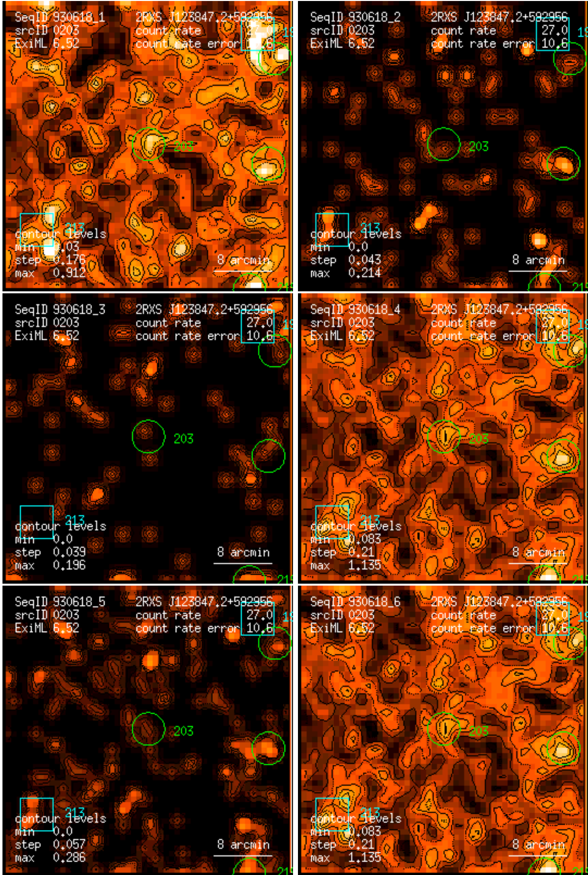
Figure 203: RASS 930618: detection 0203: band rate images, Gaussian filter: (1) PSPC channels 11 – 41, (2) 52 – 90, (3) 91 – 201, (4) 11 – 235, (5) 52 – 201, (6) 11 – 201. Broad band rates in counts/ks. Band rate contour levels in counts/ks/arcmin 2 .
