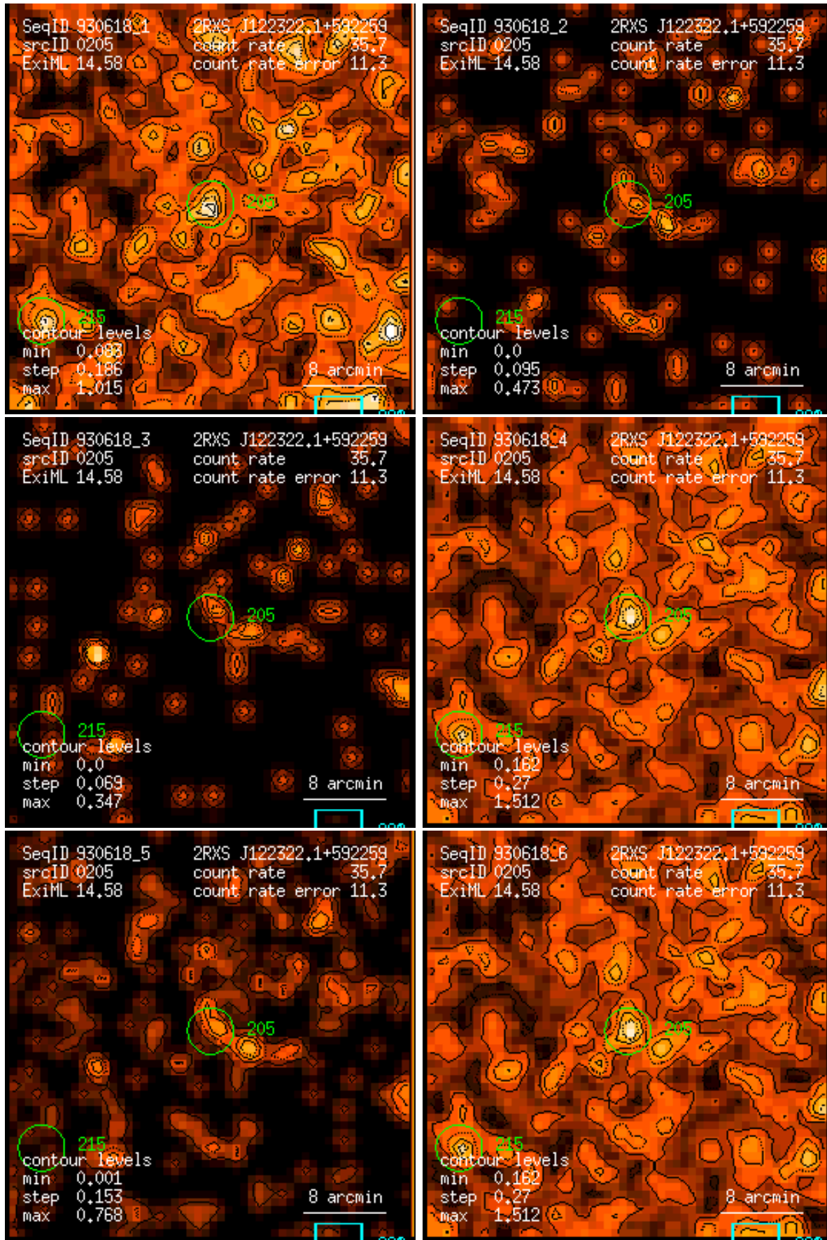
Figure 205: RASS 930618: detection 0205: band rate images, Gaussian filter: (1) PSPC channels 11 – 41, (2) 52 – 90, (3) 91 – 201, (4) 11 – 235, (5) 52 – 201, (6) 11 – 201. Broad band rates in counts/ks. Band rate contour levels in counts/ks/arcmin 2 .
