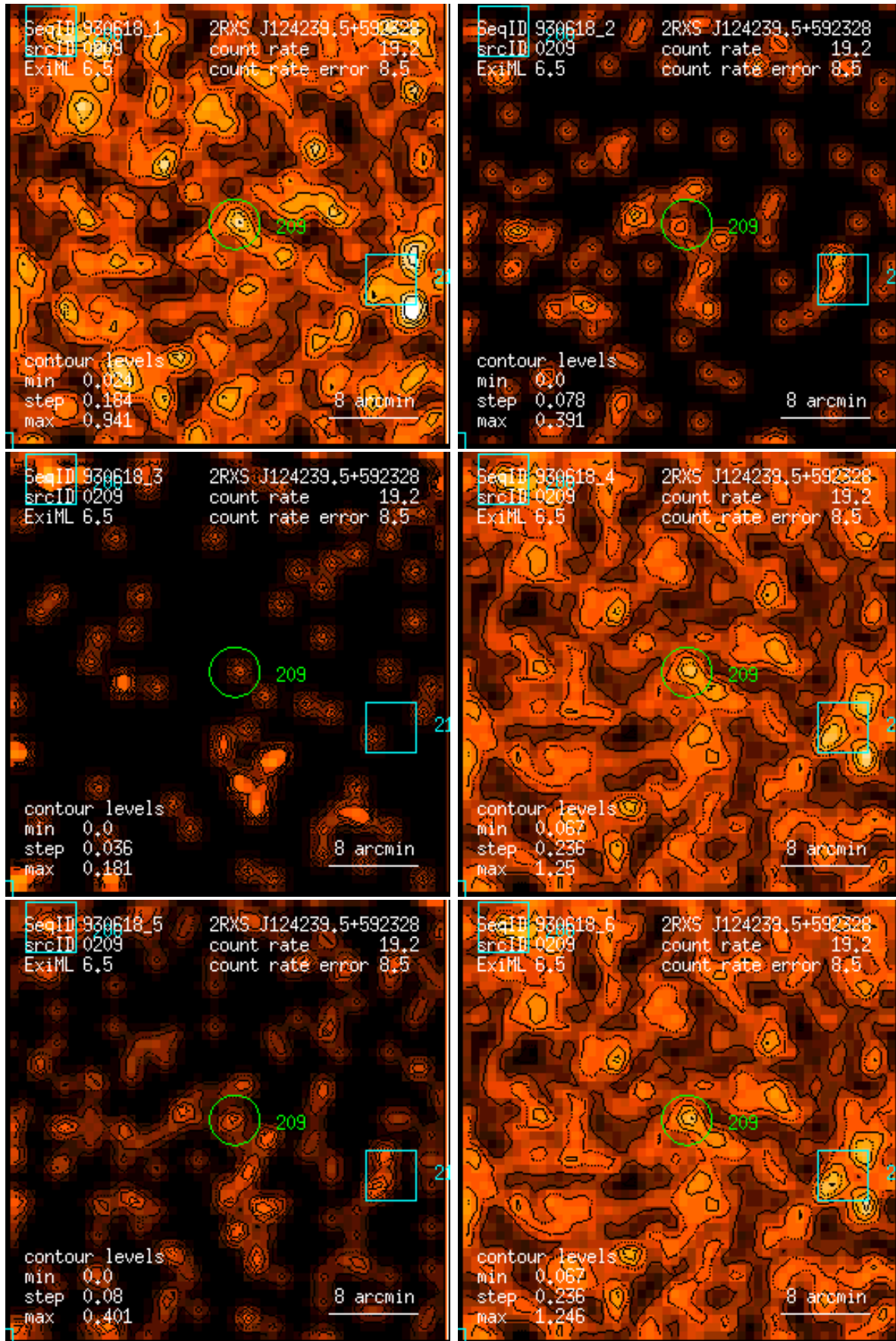
Figure 209: RASS 930618: detection 0209: band rate images, Gaussian filter: (1) PSPC channels 11 – 41, (2) 52 – 90, (3) 91 – 201, (4) 11 – 235, (5) 52 – 201, (6) 11 – 201. Broad band rates in counts/ks. Band rate contour levels in counts/ks/arcmin 2 .
