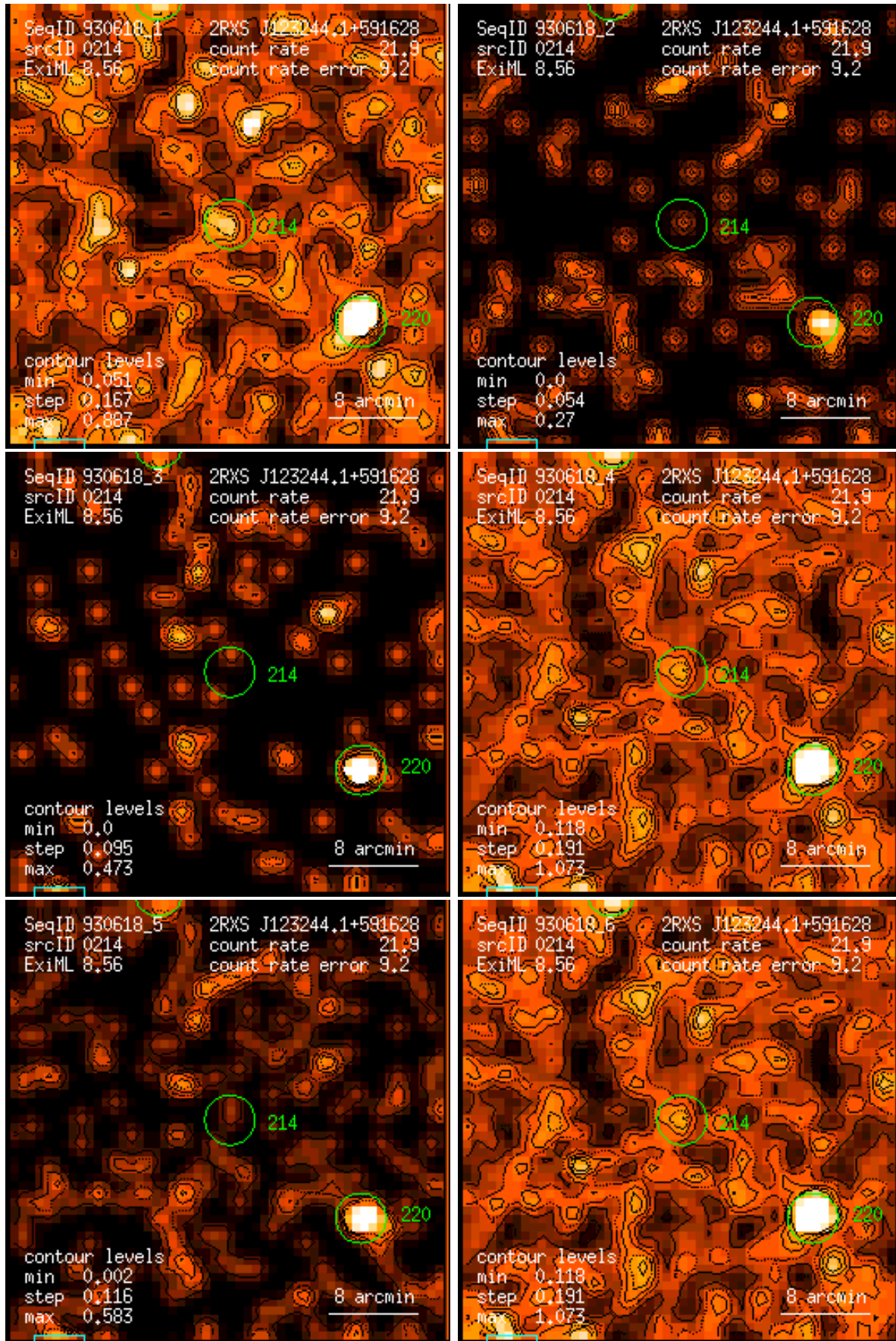
Figure 214: RASS 930618: detection 0214: band rate images, Gaussian filter: (1) PSPC channels 11 – 41, (2) 52 – 90, (3) 91 – 201, (4) 11 – 235, (5) 52 – 201, (6) 11 – 201. Broad band rates in counts/ks. Band rate contour levels in counts/ks/arcmin 2 .
