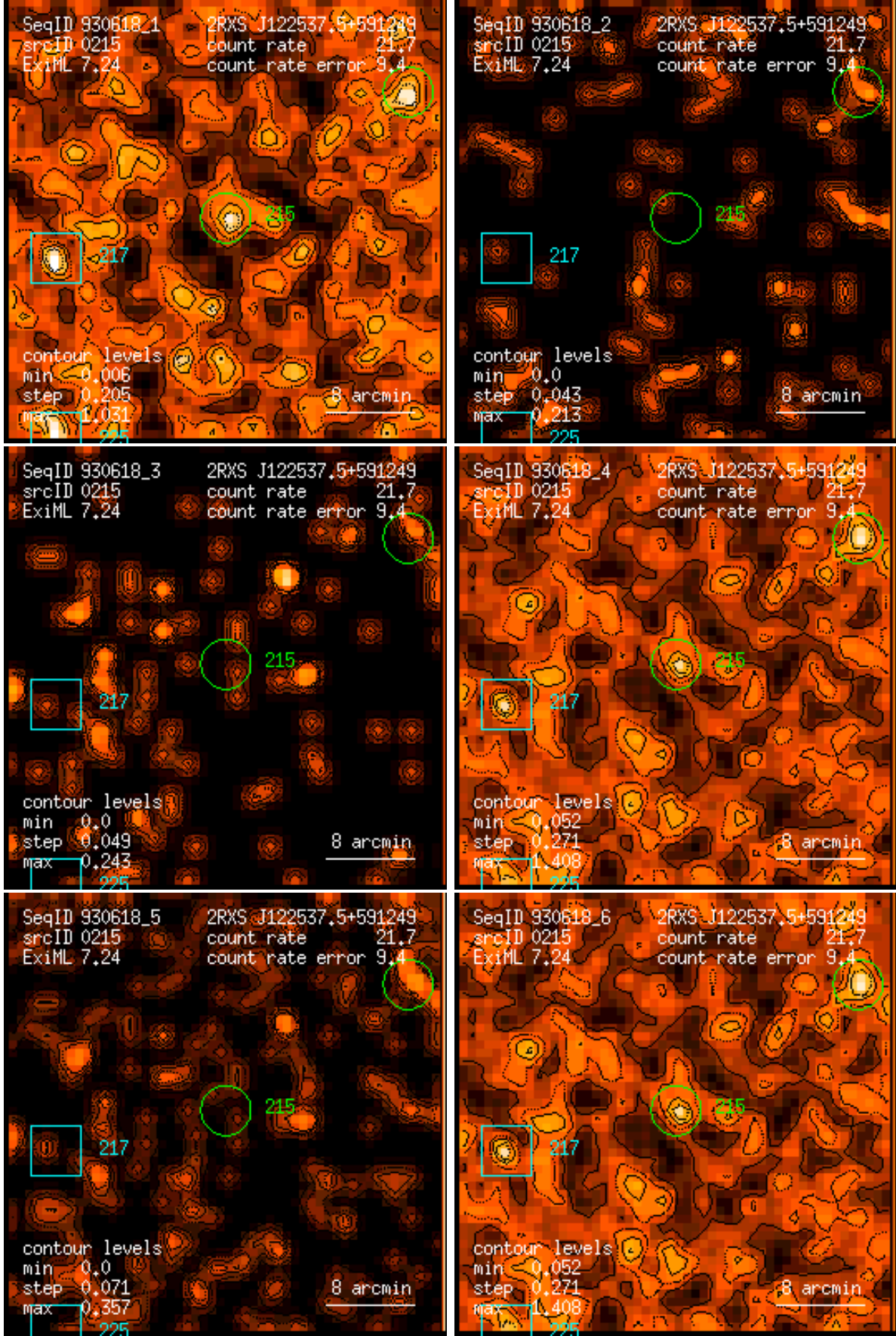
Figure 215: RASS 930618: detection 0215: band rate images, Gaussian filter: (1) PSPC channels 11 – 41, (2) 52 – 90, (3) 91 – 201, (4) 11 – 235, (5) 52 – 201, (6) 11 – 201. Broad band rates in counts/ks. Band rate contour levels in counts/ks/arcmin 2 .
