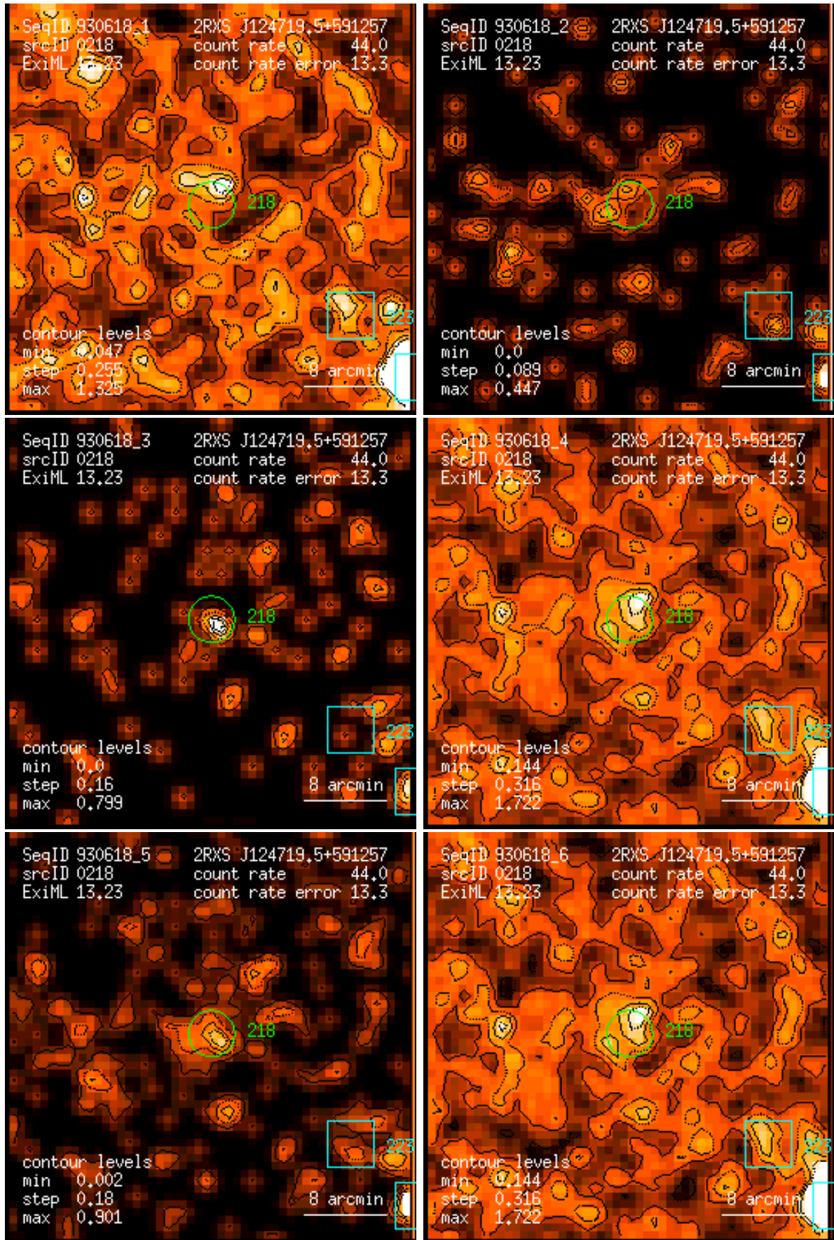
Figure 218: RASS 930618: detection 0218: band rate images, Gaussian filter: (1) PSPC channels 11 – 41, (2) 52 – 90, (3) 91 – 201, (4) 11 – 235, (5) 52 – 201, (6) 11 – 201. Broad band rates in counts/ks. Band rate contour levels in counts/ks/arcmin 2 .
