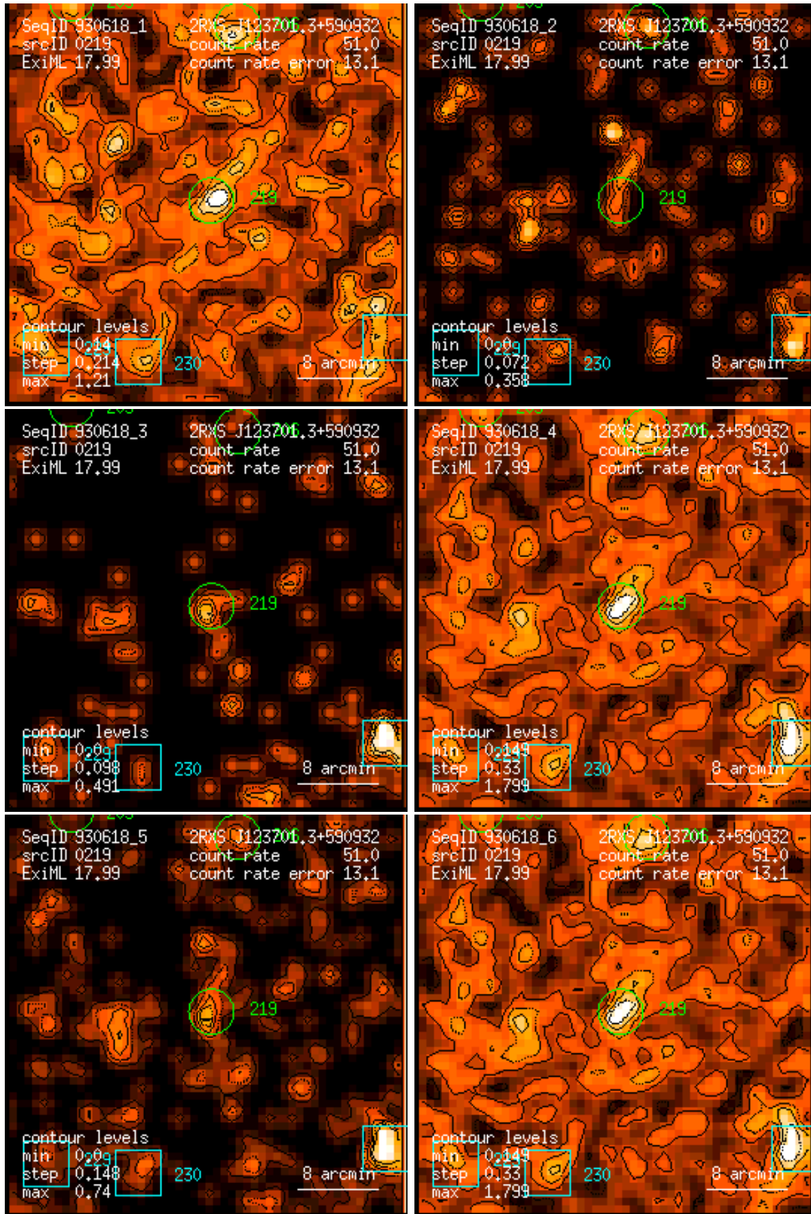
Figure 219: RASS 930618: detection 0219: band rate images, Gaussian filter: (1) PSPC channels 11 – 41, (2) 52 – 90, (3) 91 – 201, (4) 11 – 235, (5) 52 – 201, (6) 11 – 201. Broad band rates in counts/ks. Band rate contour levels in counts/ks/arcmin 2 .
