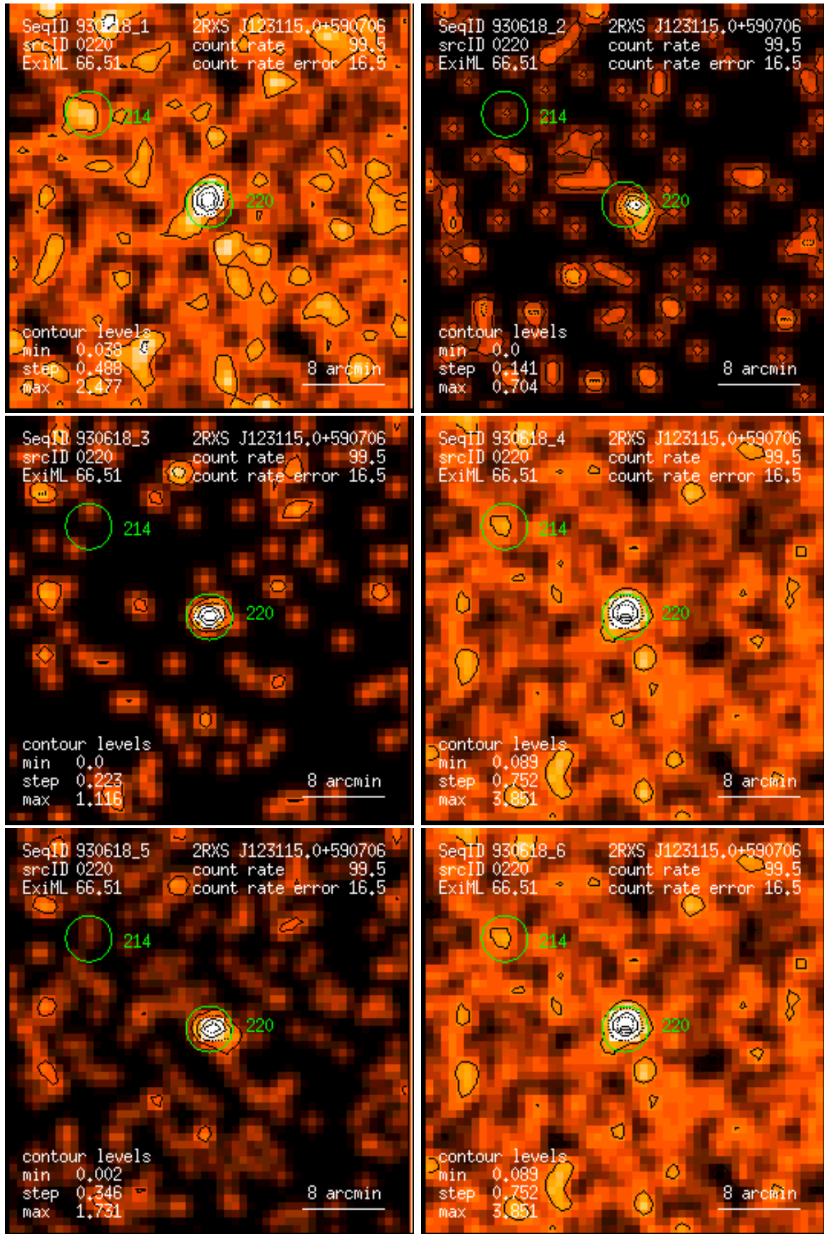
Figure 220: RASS 930618: detection 0220: band rate images, Gaussian filter: (1) PSPC channels 11 – 41, (2) 52 – 90, (3) 91 – 201, (4) 11 – 235, (5) 52 – 201, (6) 11 – 201. Broad band rates in counts/ks. Band rate contour levels in counts/ks/arcmin 2 .
