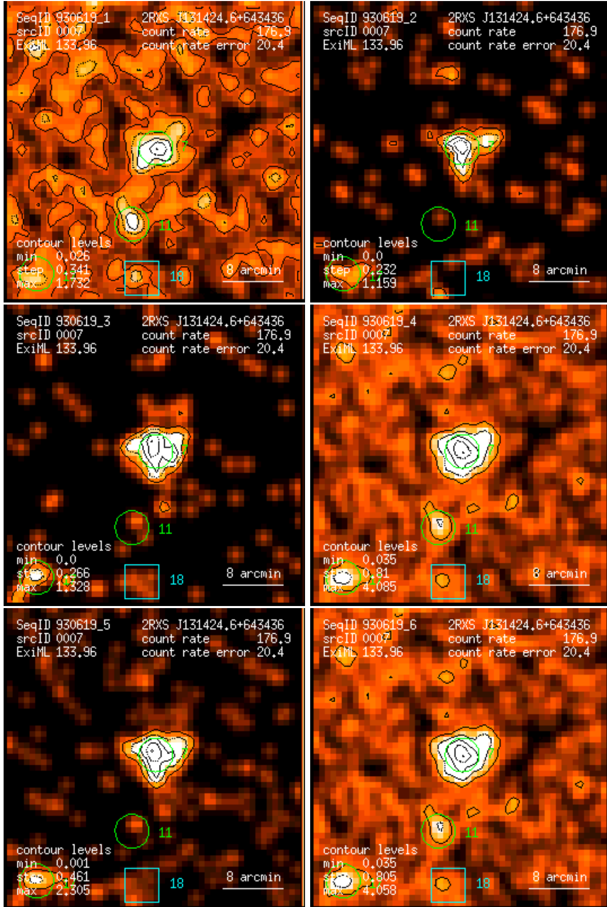
Figure 7: RASS 930619: detection 0007: band rate images, Gaussian filter: (1) PSPC channels 11 – 41, (2) 52 – 90, (3) 91 – 201, (4) 11 – 235, (5) 52 – 201, (6) 11 – 201. Broad band rates in counts/ks. Band rate contour levels in counts/ks/arcmin 2 .
