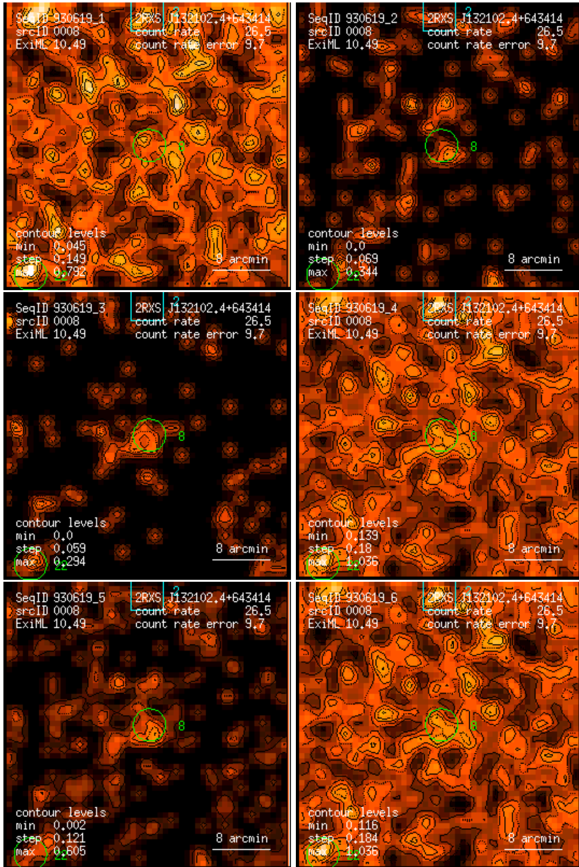
Figure 8: RASS 930619: detection 0008: band rate images, Gaussian filter: (1) PSPC channels 11 – 41, (2) 52 – 90, (3) 91 – 201, (4) 11 – 235, (5) 52 – 201, (6) 11 – 201. Broad band rates in counts/ks. Band rate contour levels in counts/ks/arcmin 2 .
