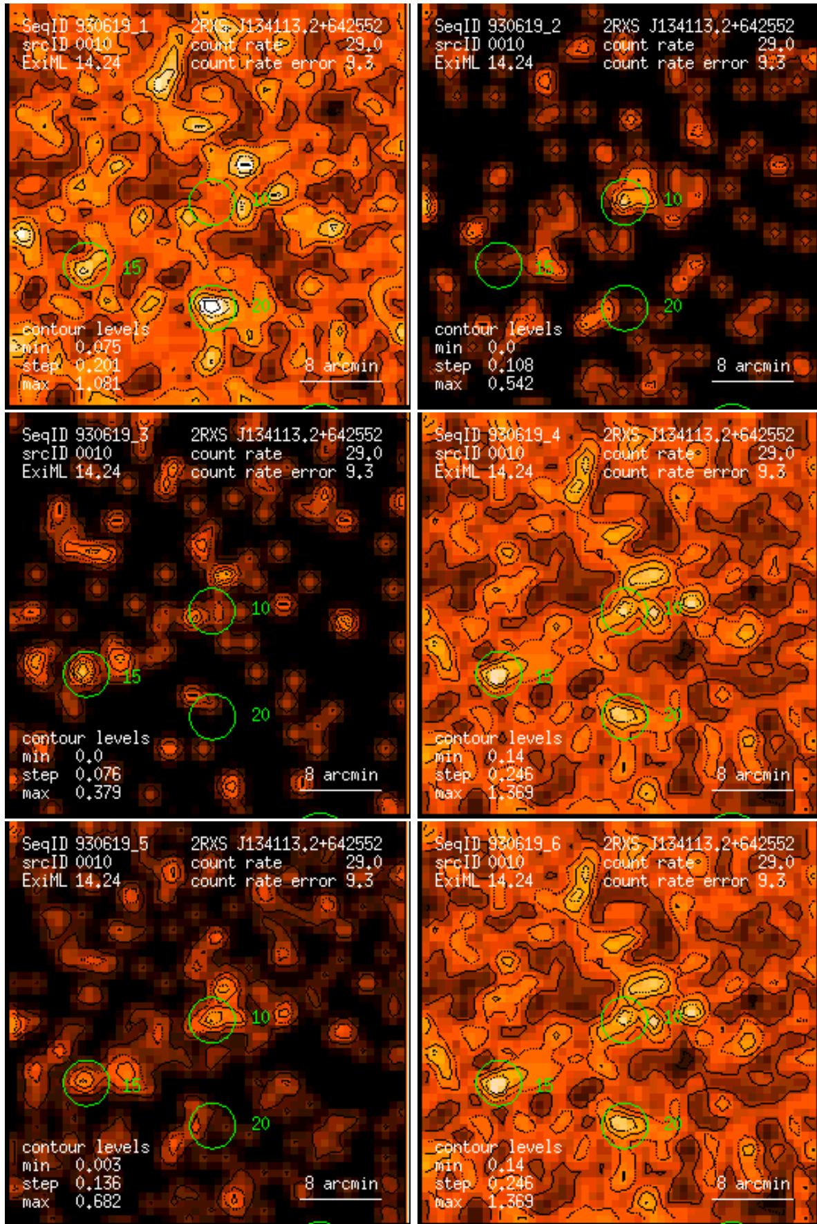
Figure 10: RASS 930619: detection 0010: band rate images, Gaussian filter: (1) PSPC channels 11 – 41, (2) 52 – 90, (3) 91 – 201, (4) 11 – 235, (5) 52 – 201, (6) 11 – 201. Broad band rates in counts/ks. Band rate contour levels in counts/ks/arcmin 2 .
